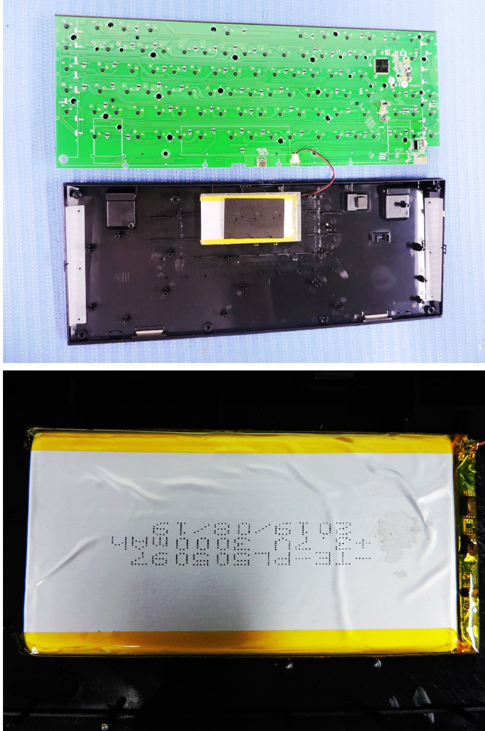
Inside view-KeyBoard
