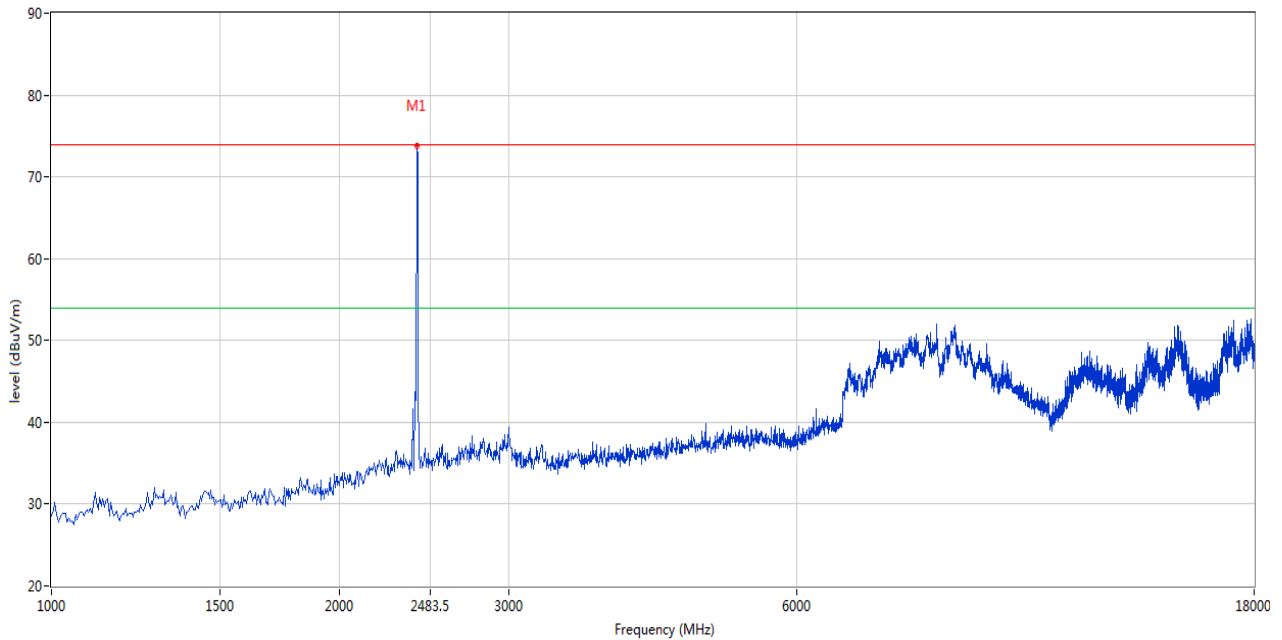
FCC Part 15B Class B 1GHz-18GHz - 2
