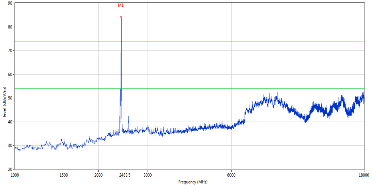
FCC_FCC Part 15B Class B 1GHz-18GHz - 2
