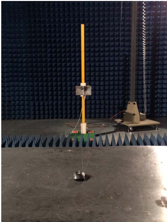
Radiated emissions test > 1GHz
