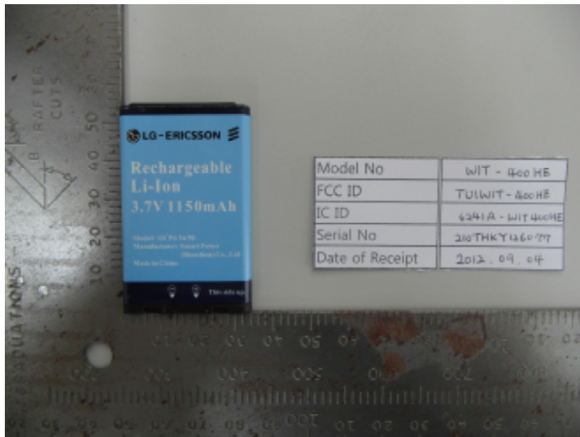
Figure 4 EUT Photo
