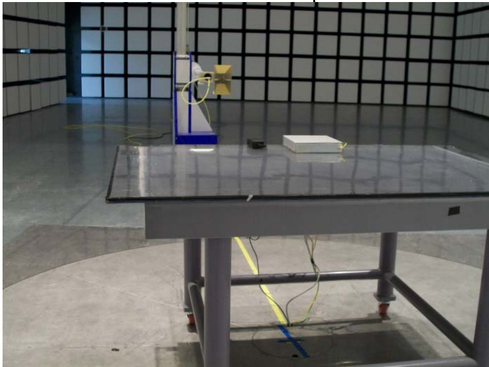
TP Mode with AC/DC Adapter
