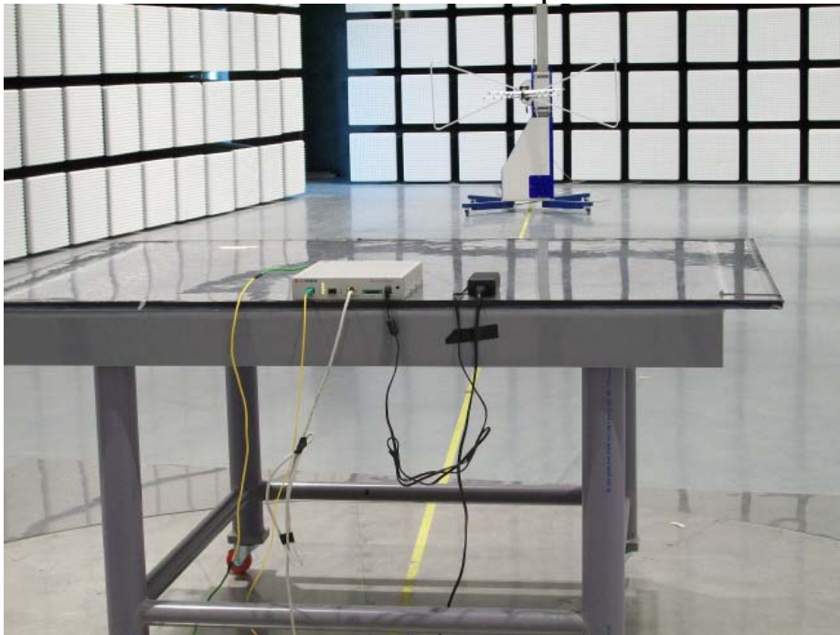
TP Mode with AC/DC Adapter
