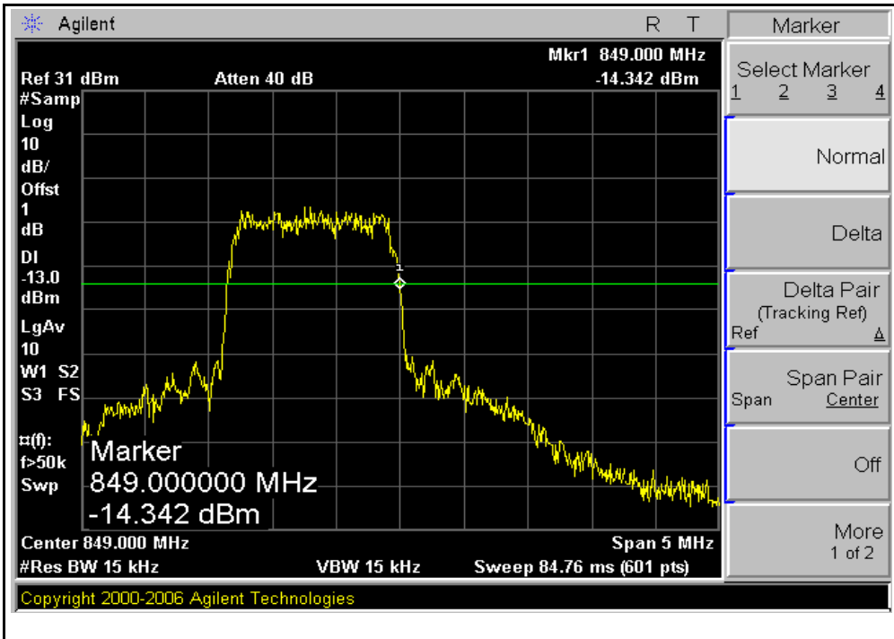
PLOTS OF EMISSION (CDMA): BAND EDGE(Ch777)
