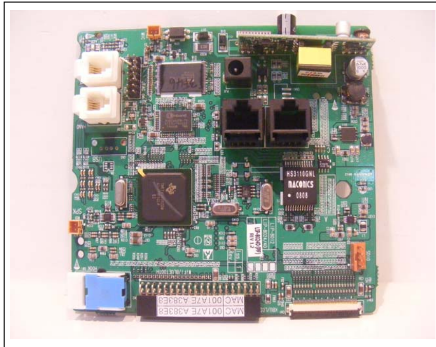
Top view of Main PCB
