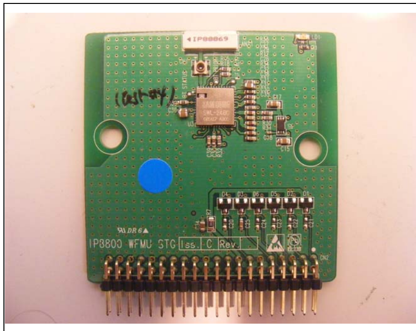
Top view of WLAN module PCB (can't remove shield cap )
