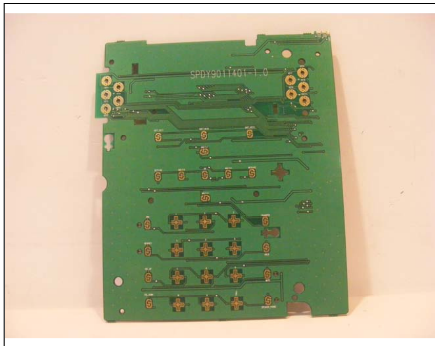
Top view of keypad PCB
