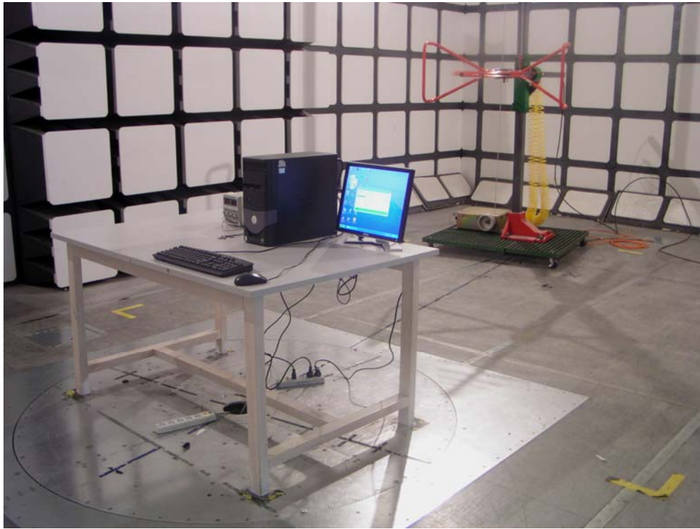
Radiated Emissions - Front View for transmitting mode (30-1000 MHz)
