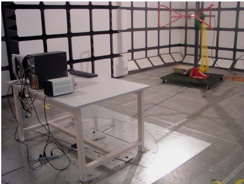
Radiated Emissions - Rear View for transmitting mode (30-1000 MHz)
