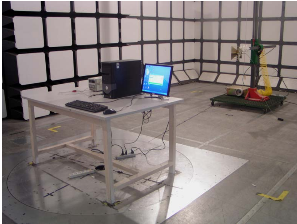
Radiated Emissions - Rear View for transmitting mode (Above 1GHz)
