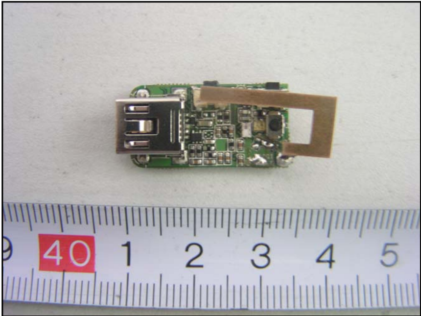
EUT – Main Board Top Components View
