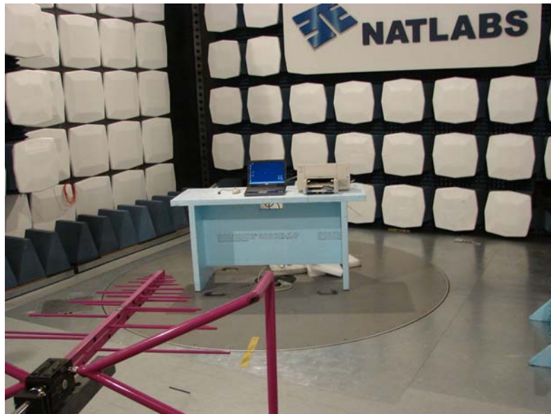
Picture 3: Receiver radiated emission measurement set-up.
