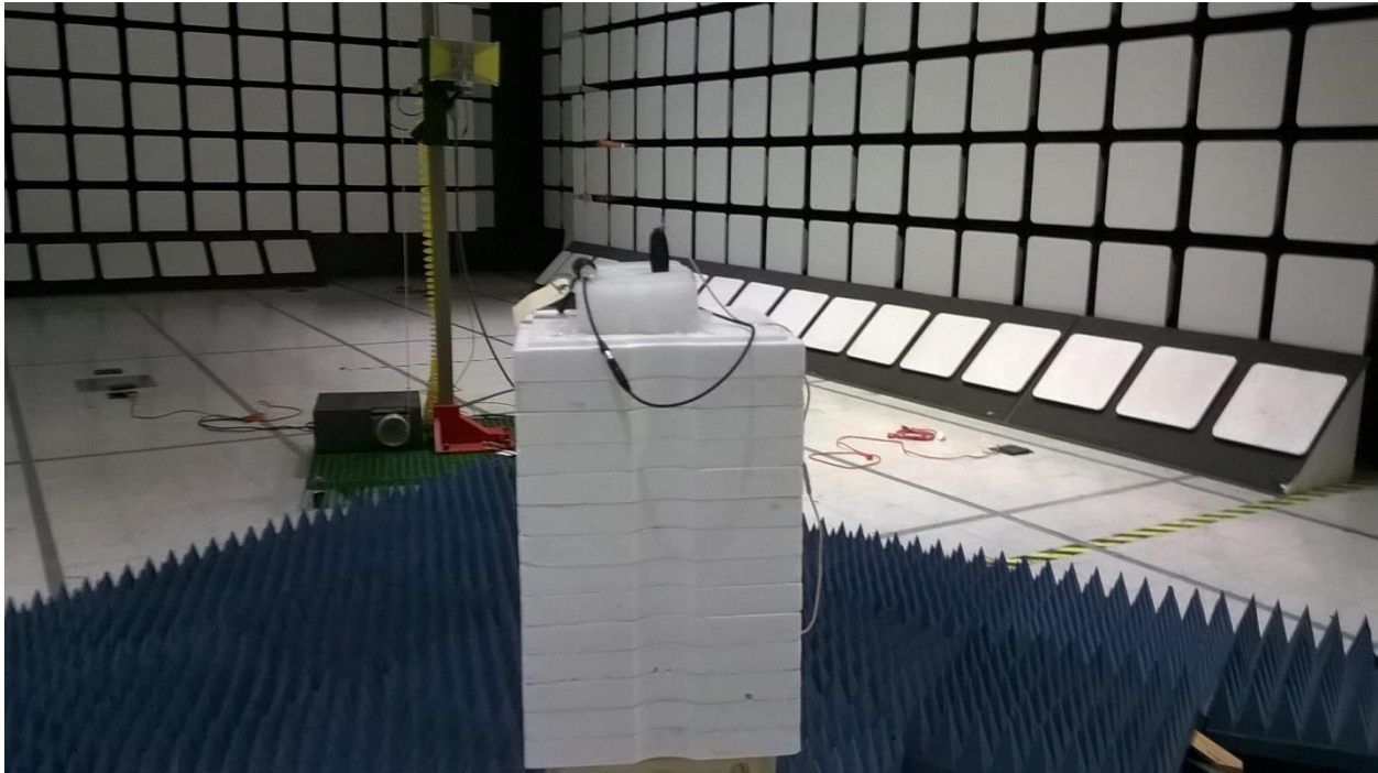
Figure 3 - Figure 1 - Radiated Emissions Test Setup, 1 - 25 GHz
