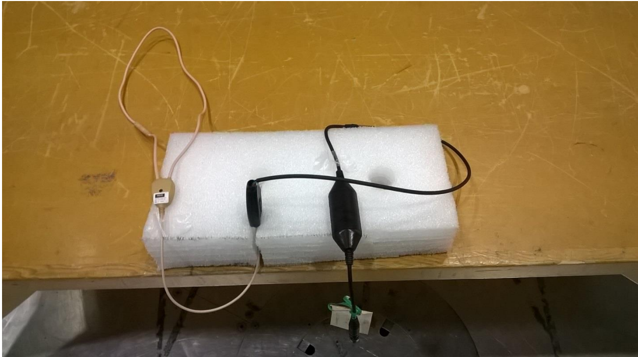
Figure 5 - Figure 1 - Radiated Emissions Test Setup, 30 MHz – 1 GHz
