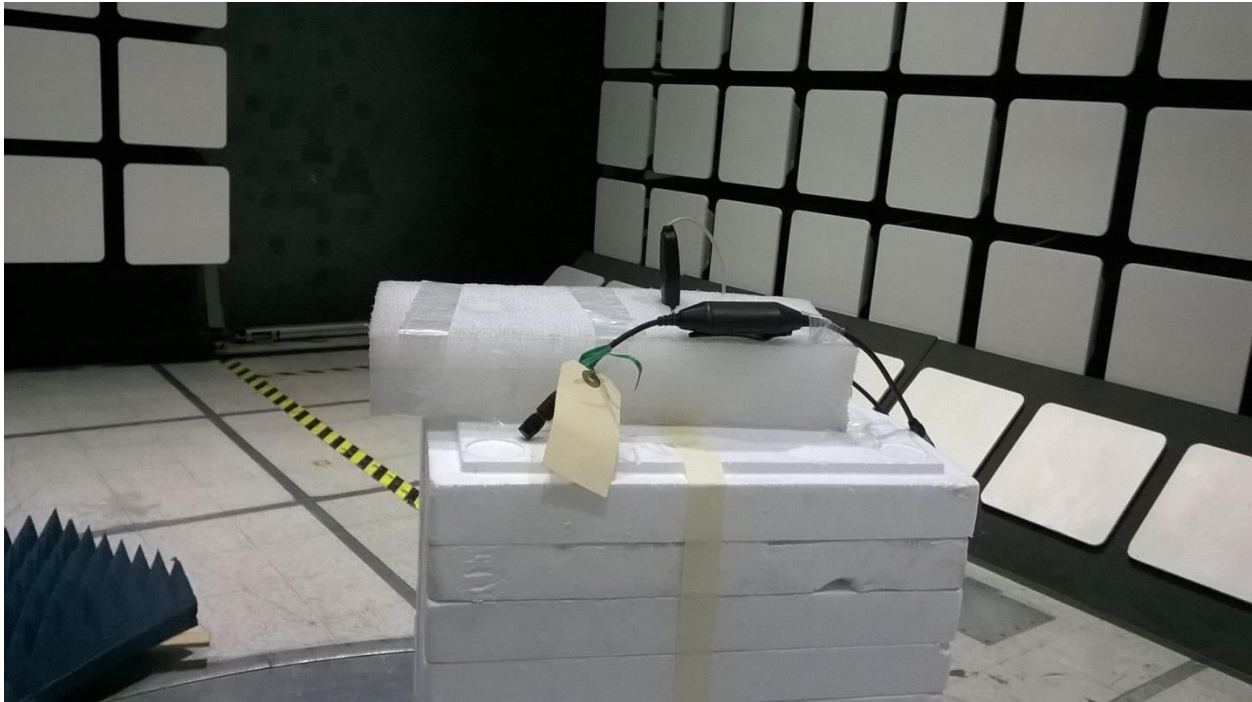
Figure 4 - Figure 1 - Radiated Emissions Test Setup, 1 - 25 GHz
