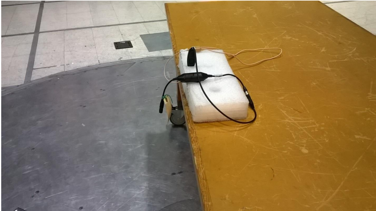
Figure 7 - Radiated Emissions Test Setup, 30 MHz – 1 GHz
