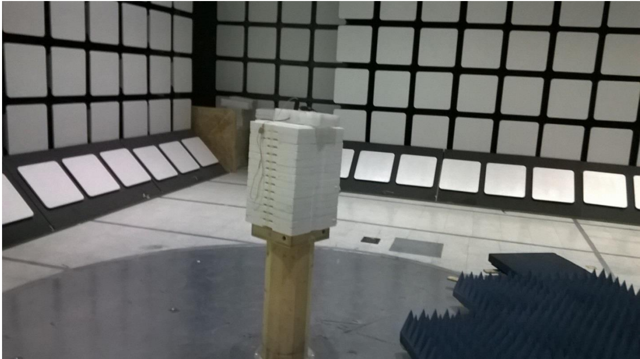
Figure 1 - Radiated Emissions Test Setup, 1 - 25 GHz
