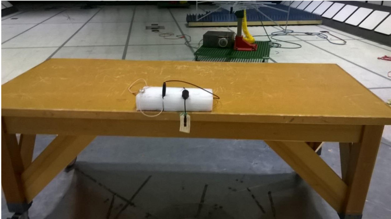
Figure 6 - Radiated Emissions Test Setup, 30 MHz – 1 GHz
