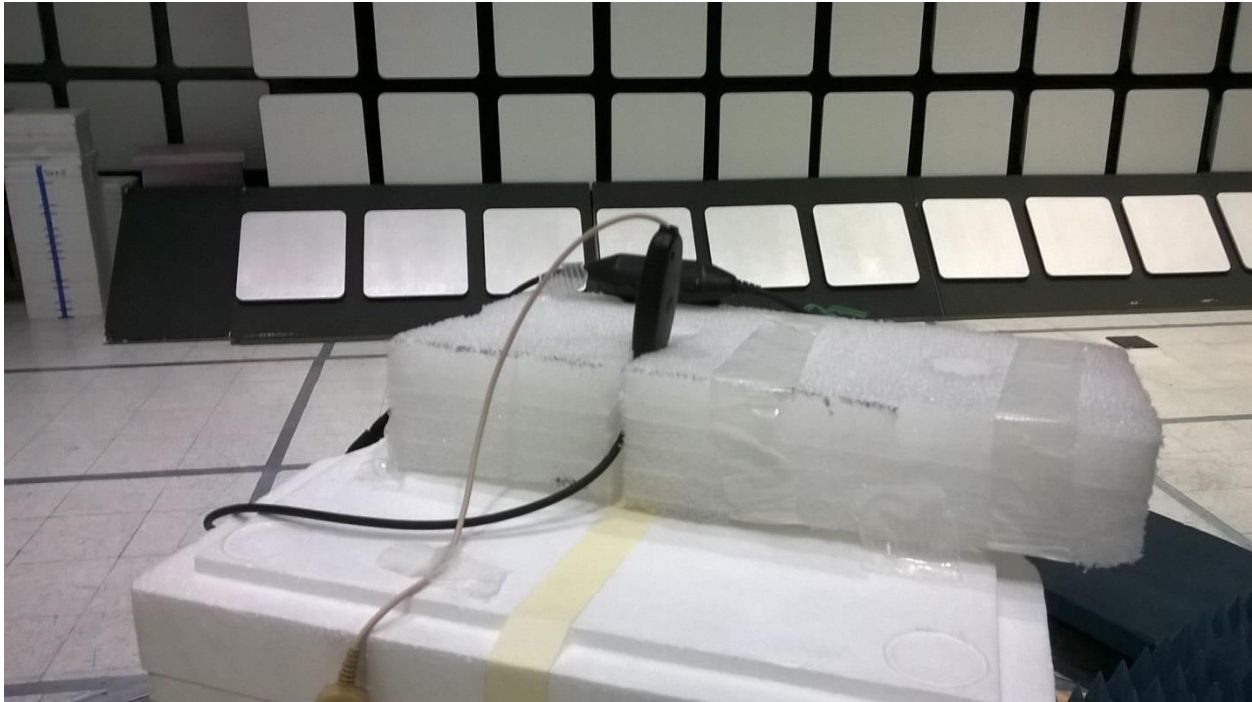
Figure 2 - Figure 1 - Radiated Emissions Test Setup, 1 - 25 GHz
