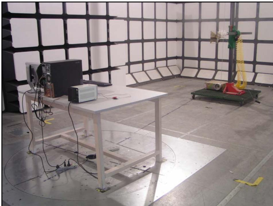
Radiated Emissions - Rear View (Above 1 GHz) for Transmitting mode
