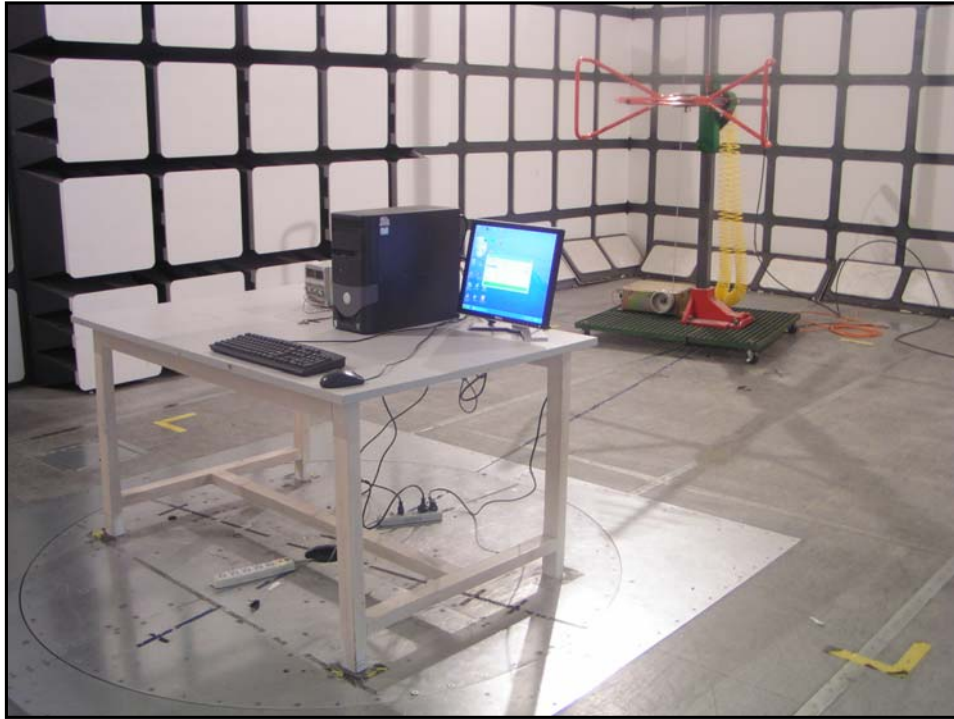
Radiated Emissions - Front View (up to 1 GHz) for Transmitting mode
