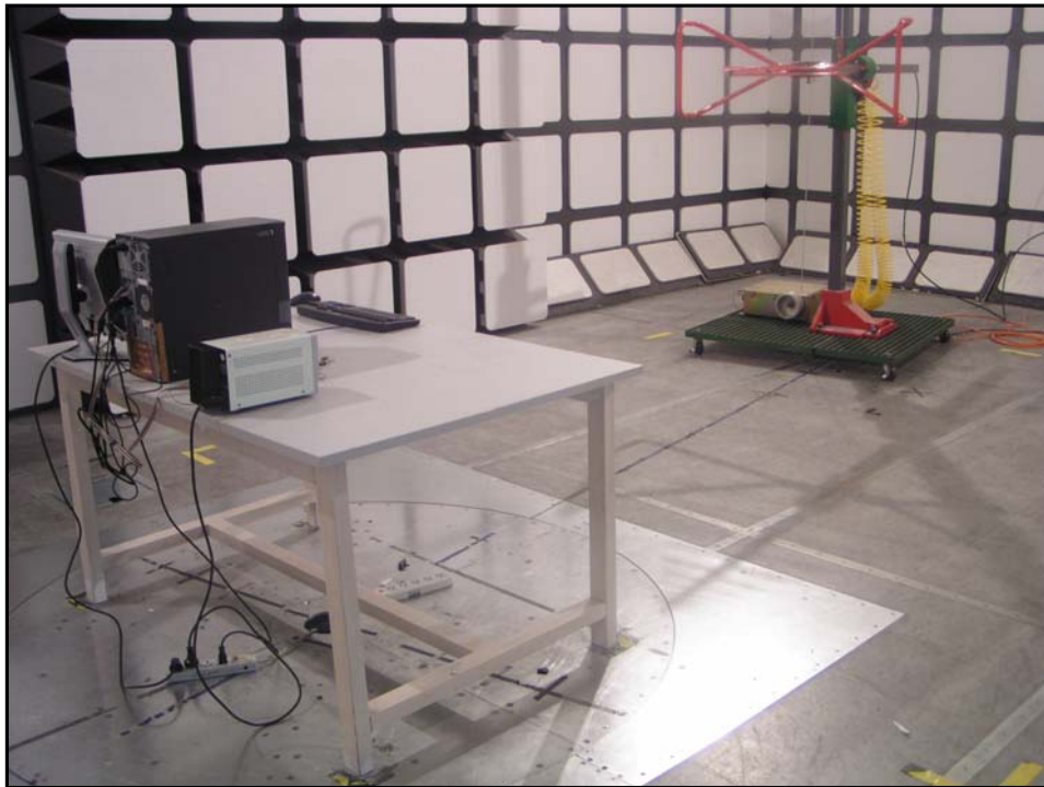
Radiated Emissions - Rear View (up to 1 GHz) for Transmitting mode
