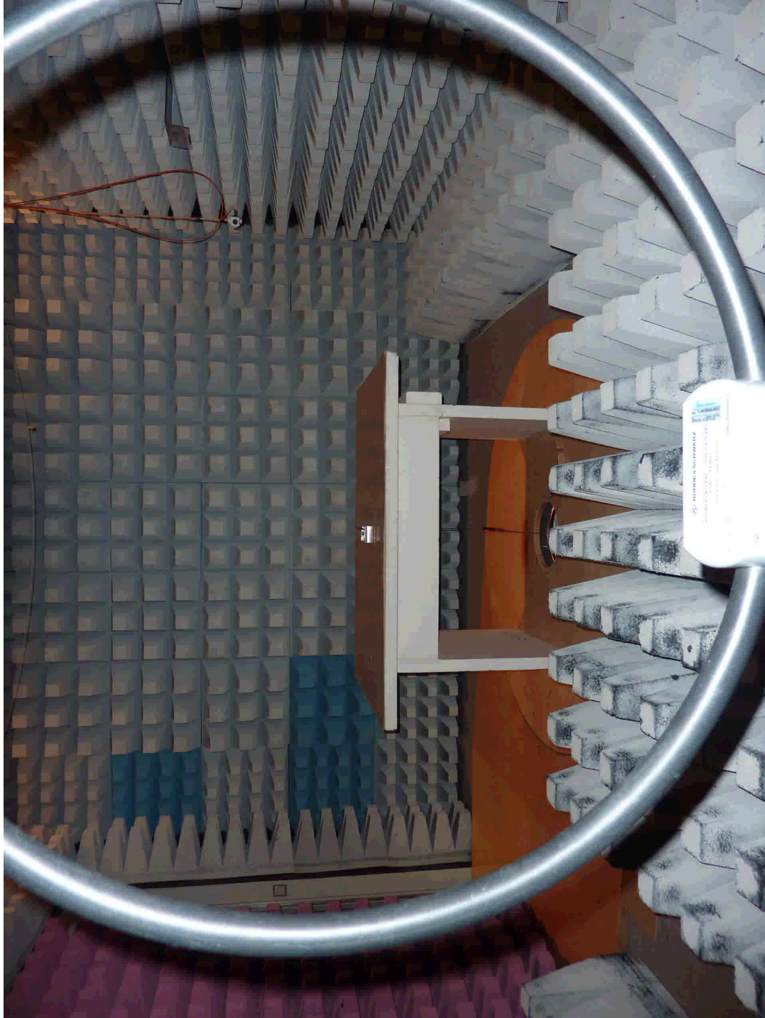
101336_10.jpg cB-OBC001i, test set-up fully anechoic chamber
