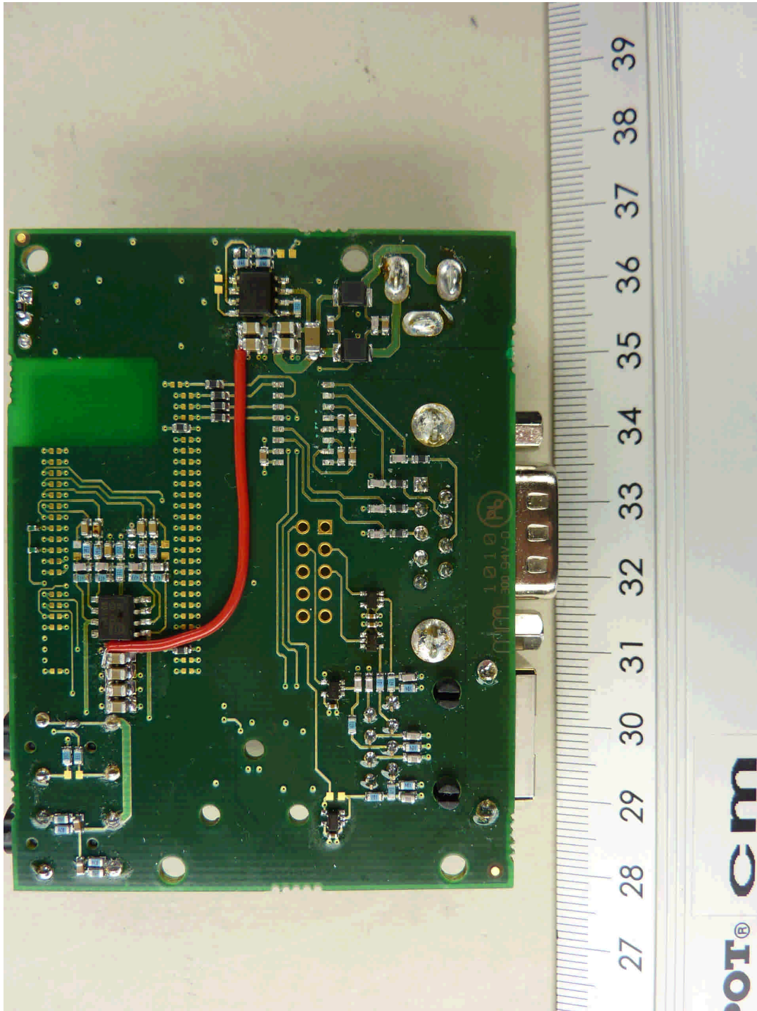
101336_f.jpg cB-OBC001i, carrier board (cB-0942), bottom view
