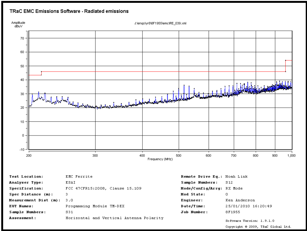
Unintentional Radiated spurious emissions 200MHz to 1GHz
