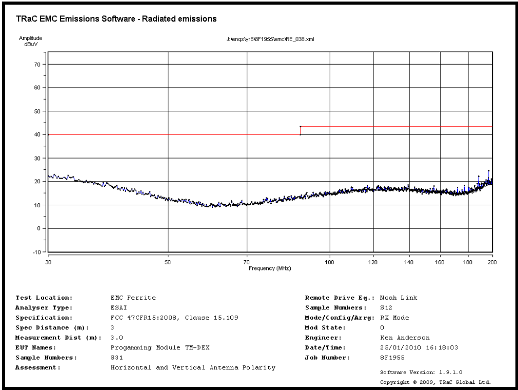
Unintentional Radiated spurious emissions 30MHz to 200MHz
