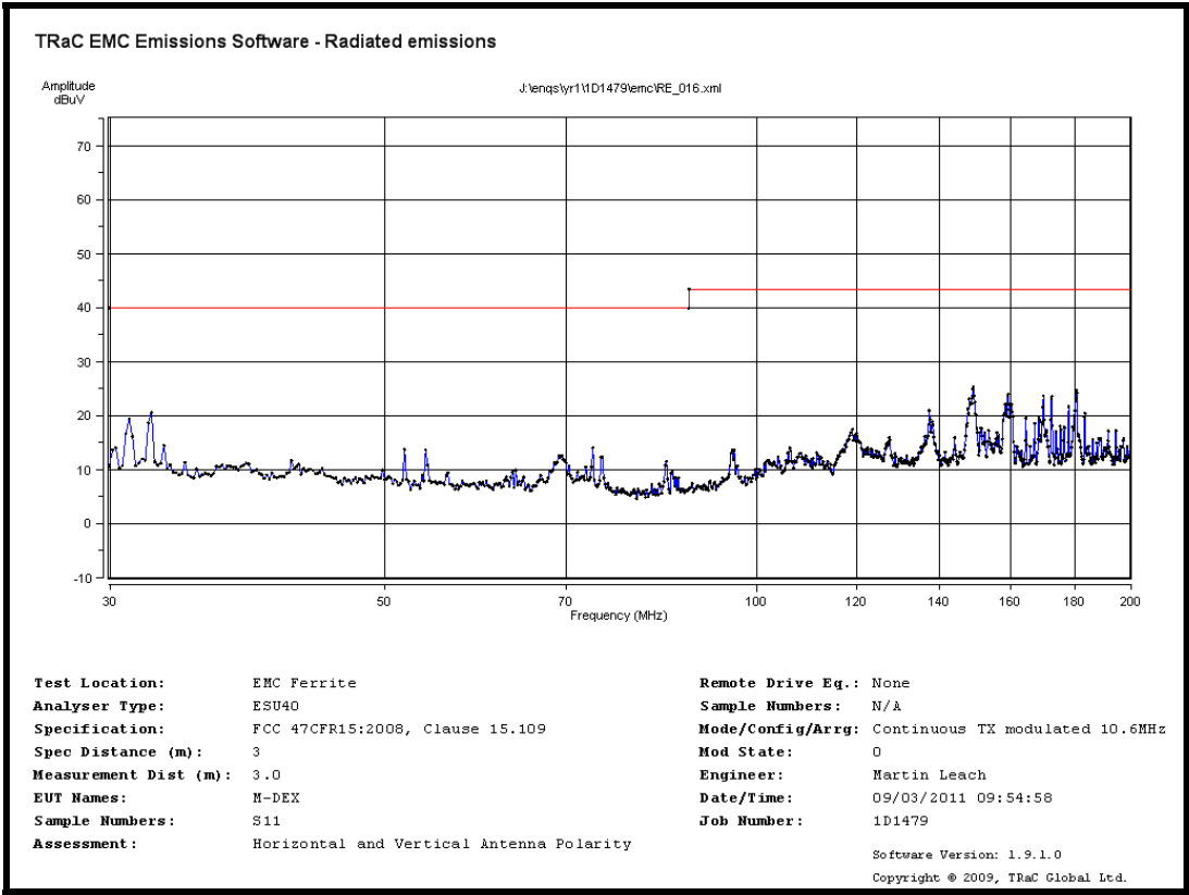
Radiated spurious emissions 30MHz - 200MHz
