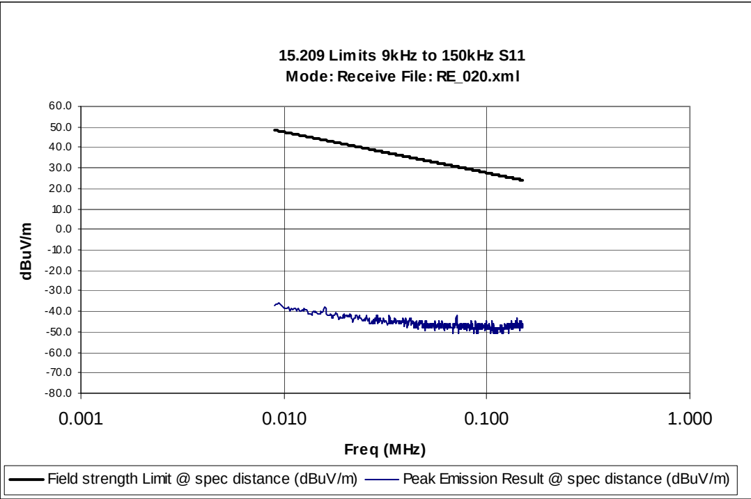
Unintentional Radiated spurious emissions 9kHz to 150kHz
