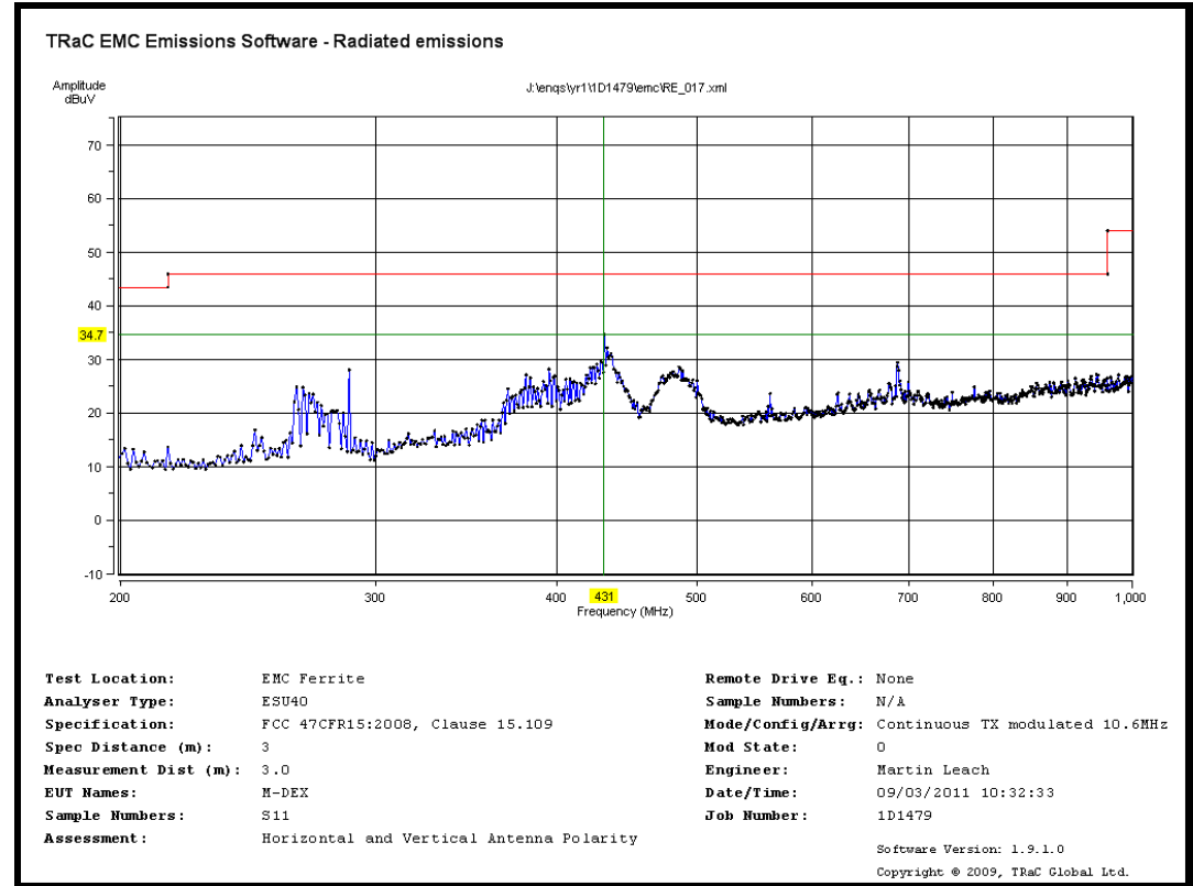
Radiated spurious emissions 200MHz - 1000MHz
