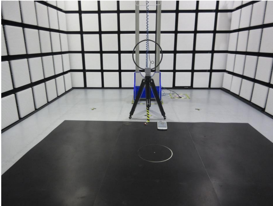
Below 30 MHz Radiated emission
