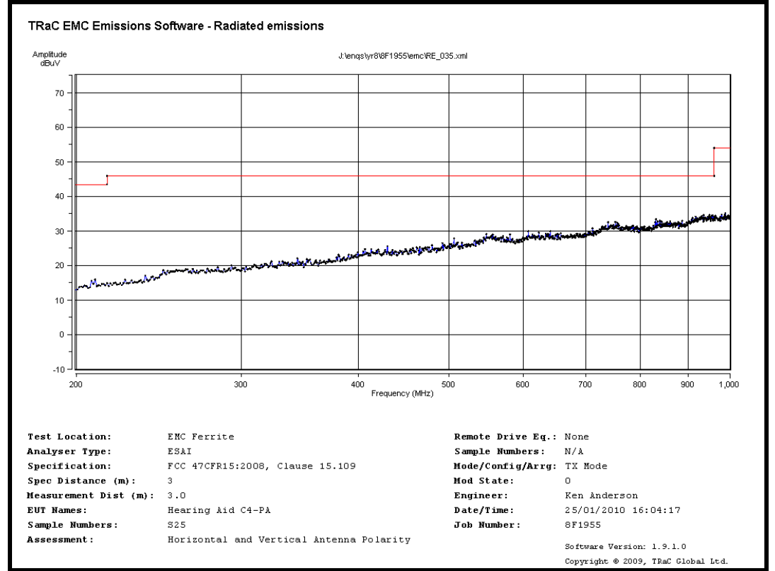
Radiated spurious emissions 200MHz to 1GHz
