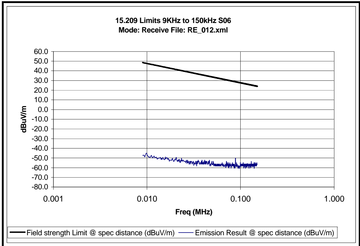
Unintentional Radiated spurious emissions 9kHz to 150kHz
