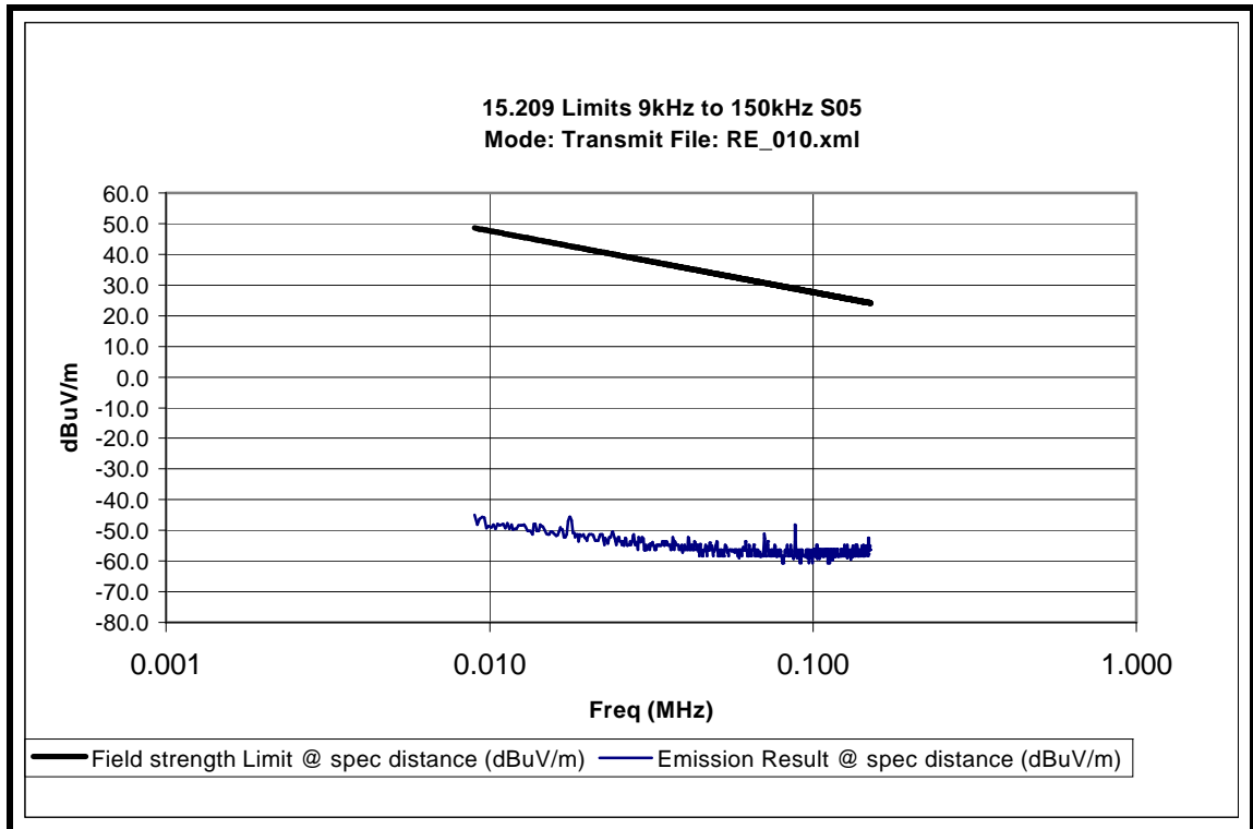
Radiated spurious emissions 9kHz to 150kHz
