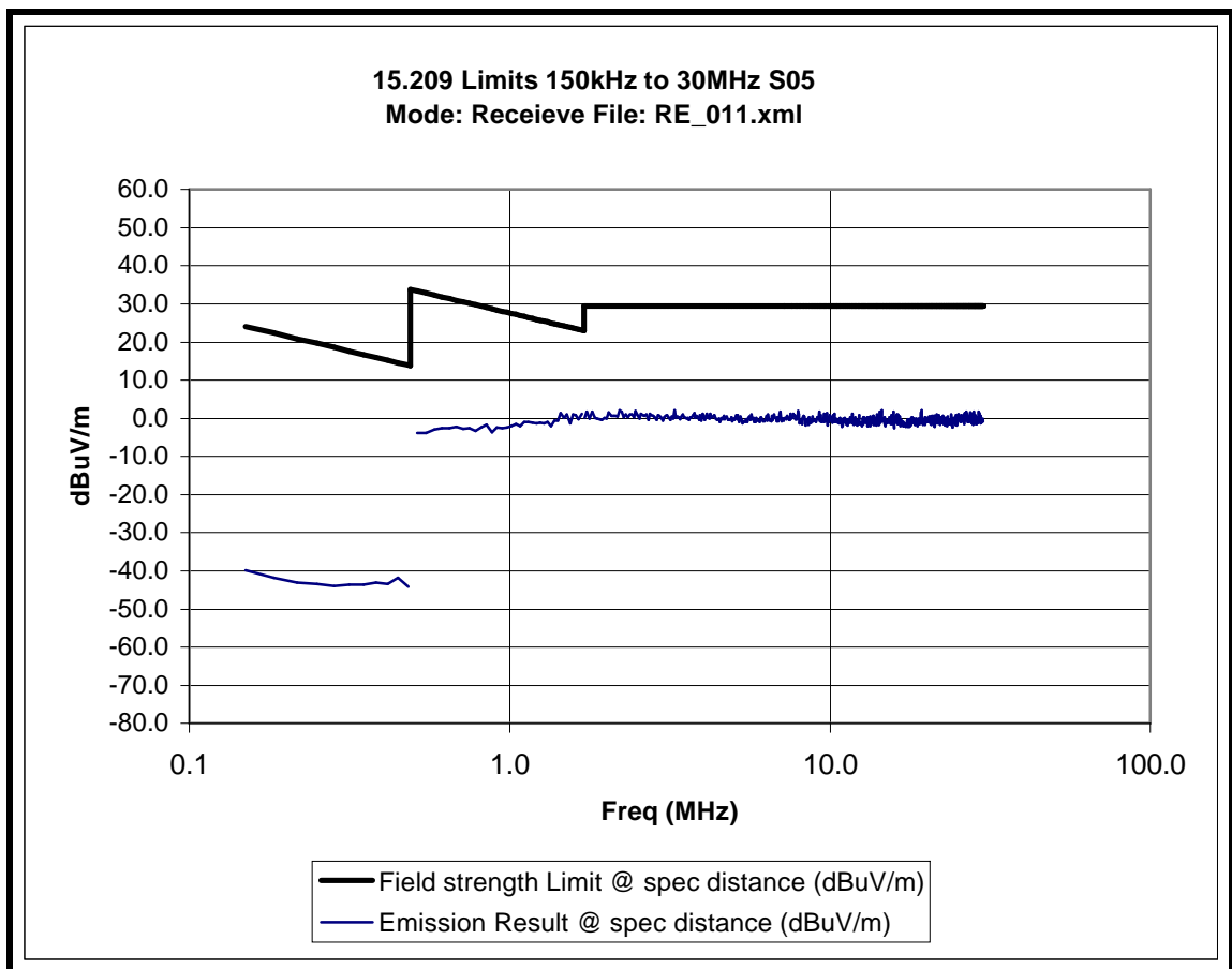
Radiated spurious emissions 150kHz to 30MHz
