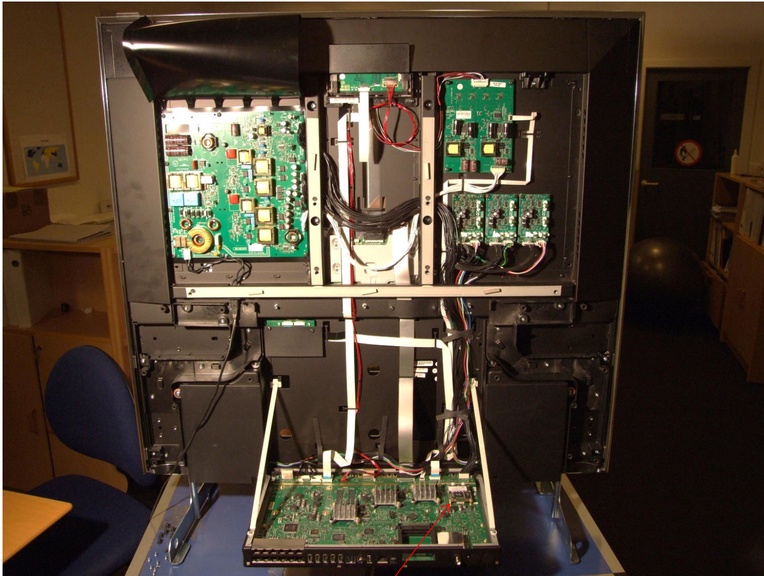
Full view Video Engine in BeoVision 11 in service mode with LBWA1ZZPD
