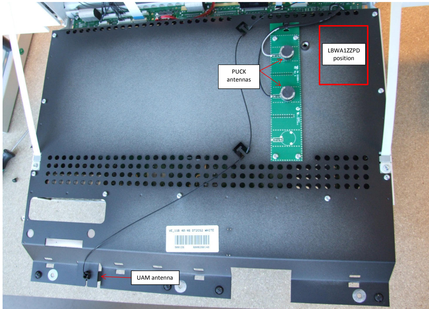
Video Engine with cover on, placed in BeoVision 11 with Antennas: PUCK and UAM
