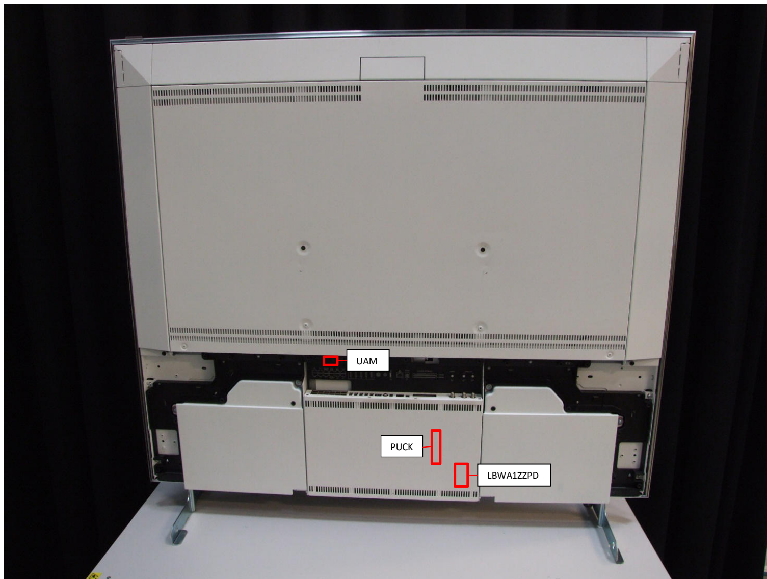
BeoVision 11 with indication of LBWA1ZZPD and antennas normal operating position.
