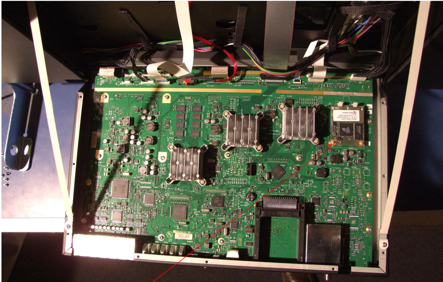
Close up Video Engine with LBWA1ZZPD
