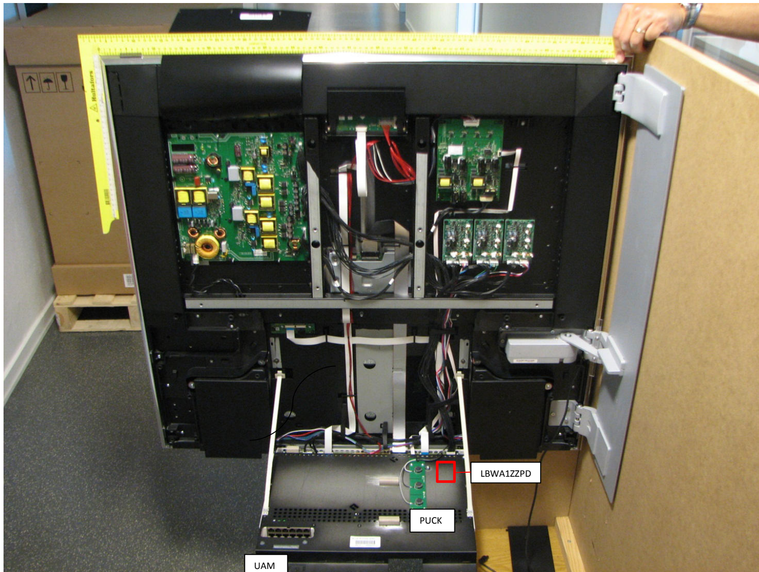
BeoVision 11 Video Engine and LBWA1ZZPD and antennas PUCK and UAM
