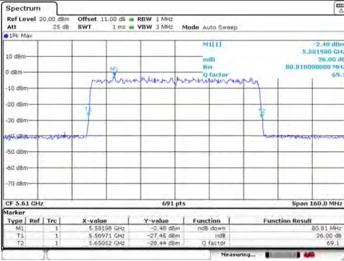
26dB Bandwidth
