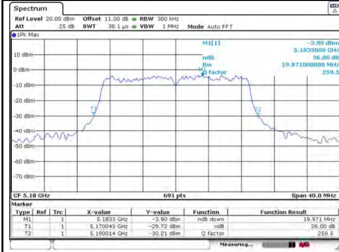
26dB Bandwidth
