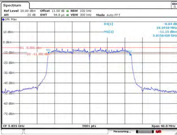
6dB Bandwidth
