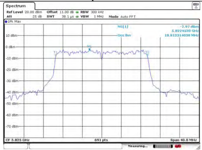
99% Occupied Bandwidth
