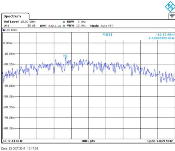
Channel 19 / 2440 MHz
