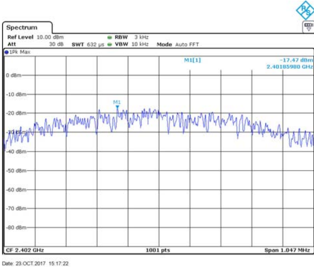
Channel 0 / 2402 MHz
