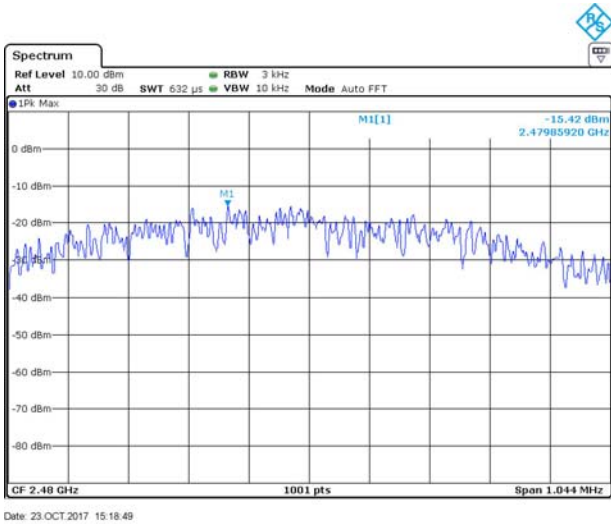
Channel 39 / 2480 MHz
