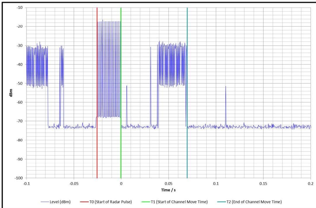
Channel Move Time 5520 MHz – Short Radar (Type 1) – First 200 ms
