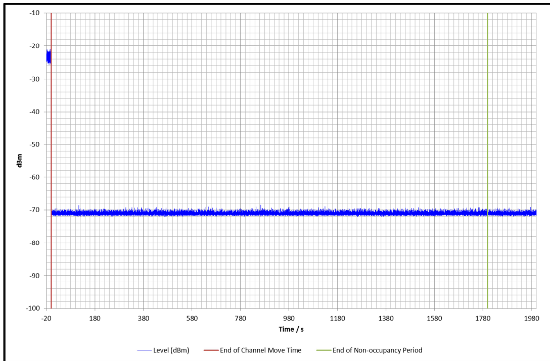
Non-occupancy Period – 5540 MHz
