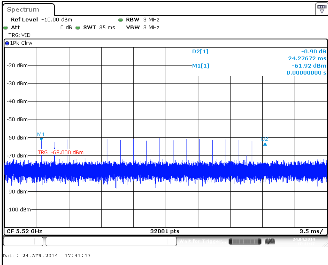
Type 1 (Short) Radar
