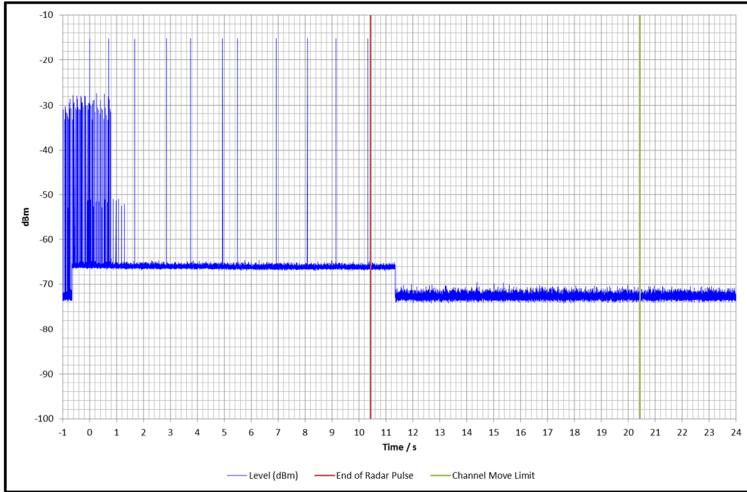
Channel Move Time 5320 MHz – Long Radar (Type 5)
