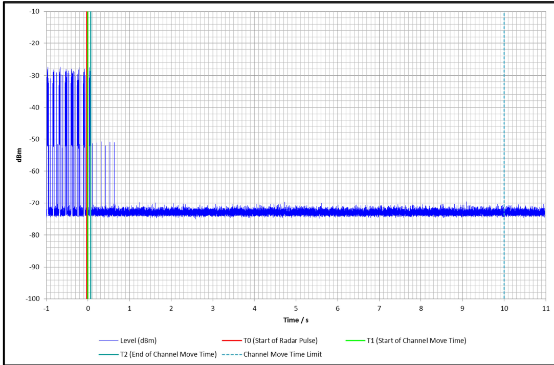
Channel Move Time 5520 MHz – Short Radar (Type 1) - Full 10 seconds
