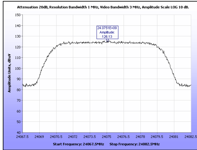
Plot 6. Radiated Field Strength of Fundamental, 10 MHz, Low Channel
