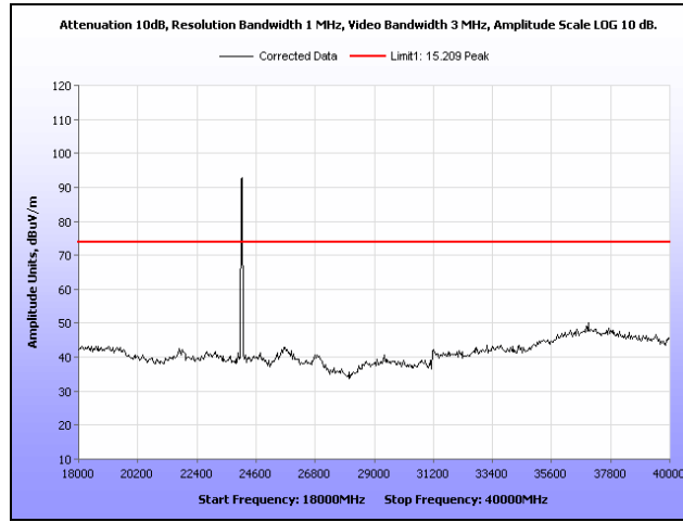
Plot 75. Radiated Spurious Emissions, 20 MHz, Low Channel, 18 GHz - 40 GHz, Peak
