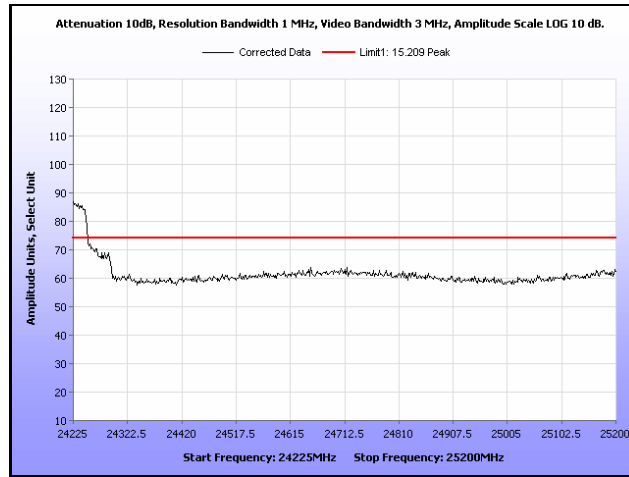
Plot 220. Radiated Band Edge, 50 MHz, High Channel, Peak
