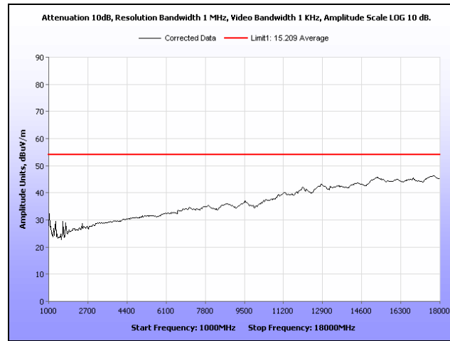
Plot 58. Radiated Spurious Emissions, 10 MHz, Mid Channel, 1 GHz – 18 GHz, Average
