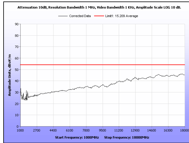
Plot 82. Radiated Spurious Emissions, 20 MHz, Mid Channel, 1 GHz – 18 GHz, Average
