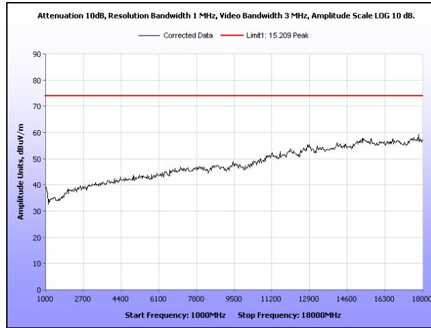
Plot 90. Radiated Spurious Emissions, 20 MHz, High Channel, 1 GHz – 18 GHz, Peak
