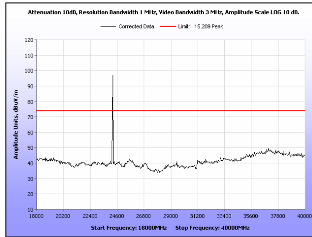
Plot 67. Radiated Spurious Emissions, 10 MHz, High Channel, 18 GHz - 40 GHz, Peak
