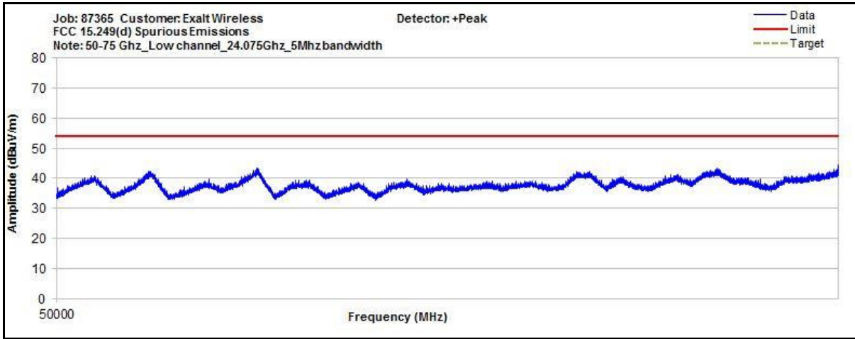
Plot 30. Radiated Spurious Emissions, 5 MHz, Low Channel, 50 GHz – 75 GHz
