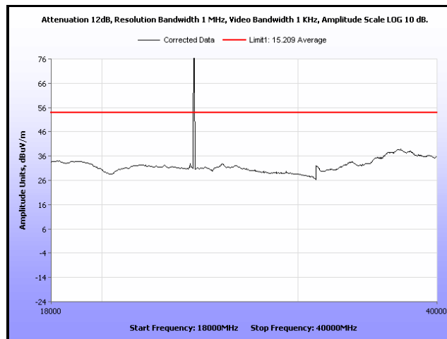
Plot 35. Radiated Spurious Emissions, 5 MHz, Mid Channel, 18 GHz – 40 GHz, Average
