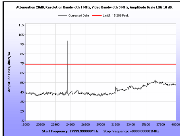
Plot 28. Radiated Spurious Emissions, 5 MHz, Low Channel, 18 GHz – 40 GHz, Peak
