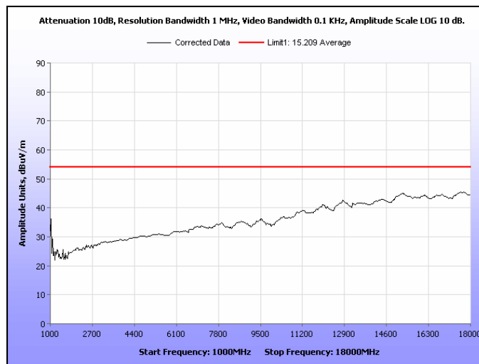
Plot 34. Radiated Spurious Emissions, 5 MHz, Mid Channel, 1 GHz – 18 GHz, Average
