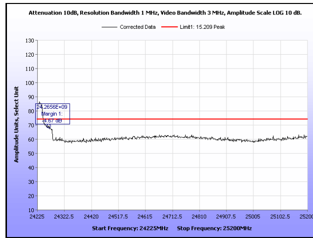
Plot 216. Radiated Band Edge, 40 MHz, High Channel, Peak
