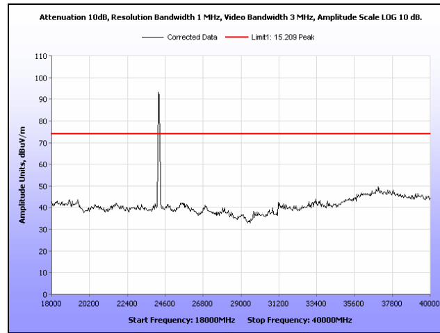
Plot 188. Radiated Spurious Emissions, 50 MHz, High Channel, 18 GHz - 40 GHz, Peak
