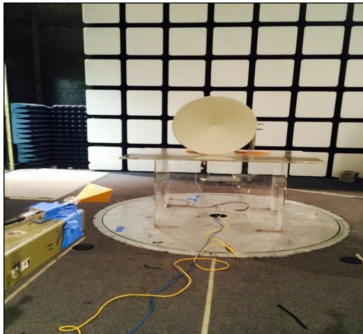
Photograph 7. Radiated Spurious Emissions, Test Setup, Above 40 GHz
