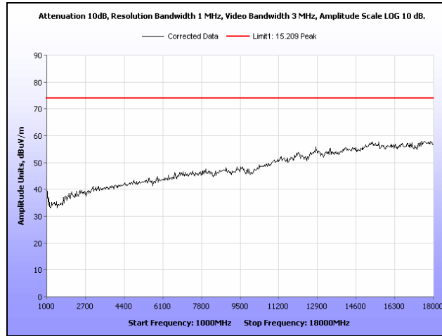
Plot 178. Radiated Spurious Emissions, 50 MHz, Mid Channel, 1 GHz - 18 GHz, Peak
