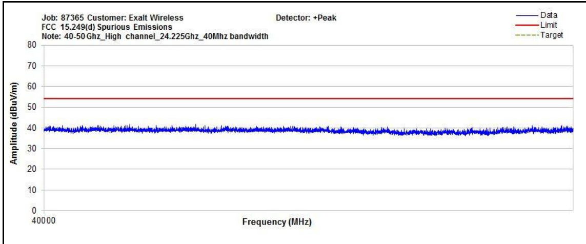
Plot 166. Radiated Spurious Emissions, 40 MHz, High Channel, 40 GHz – 50 GHz
