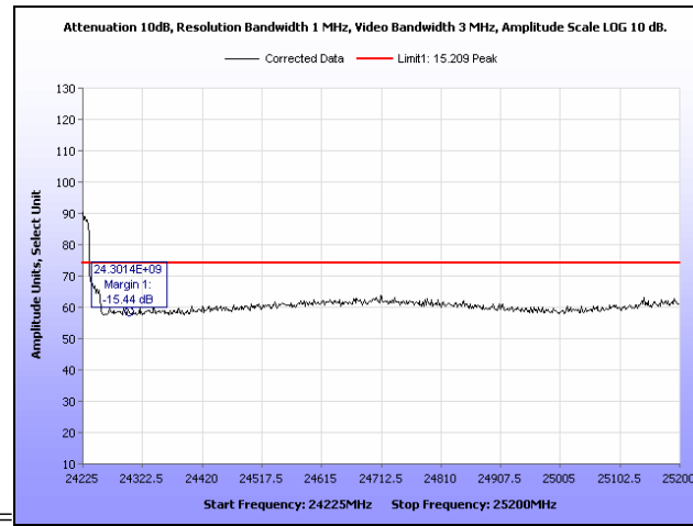
Plot 204. Radiated Band Edge, 20 MHz, High Channel, Peak
