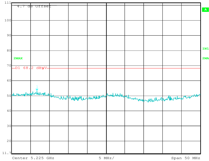
Low Channel (32MHz Mode 3)
