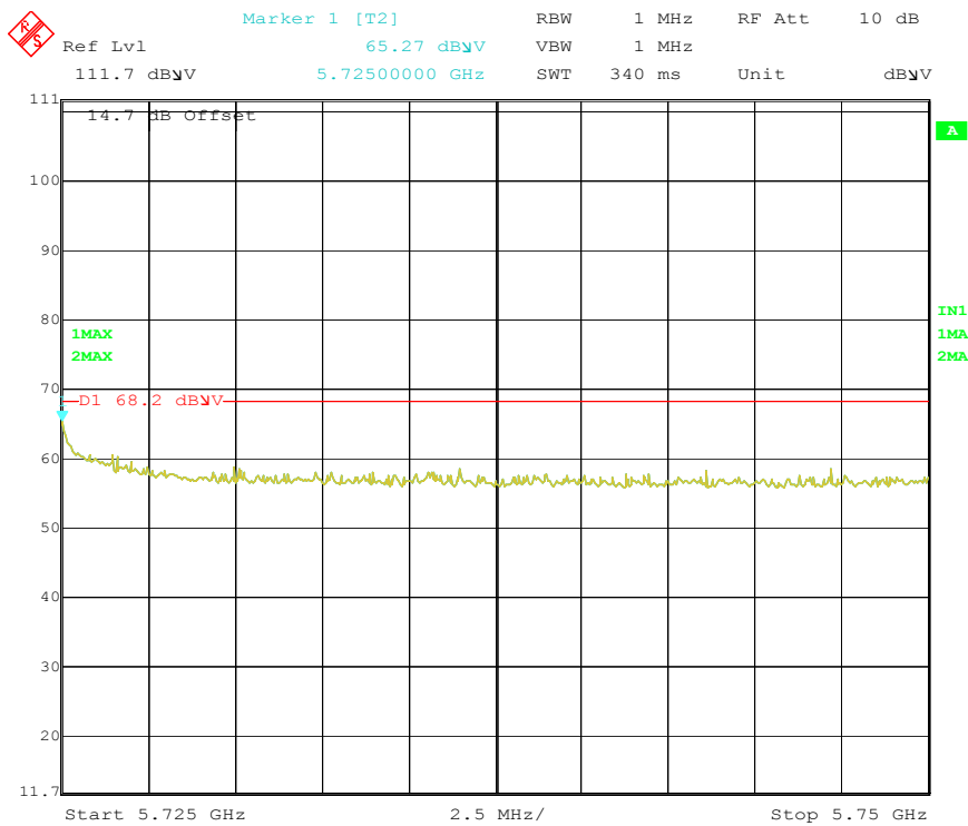
High Channel (16MHz Mode 3)
