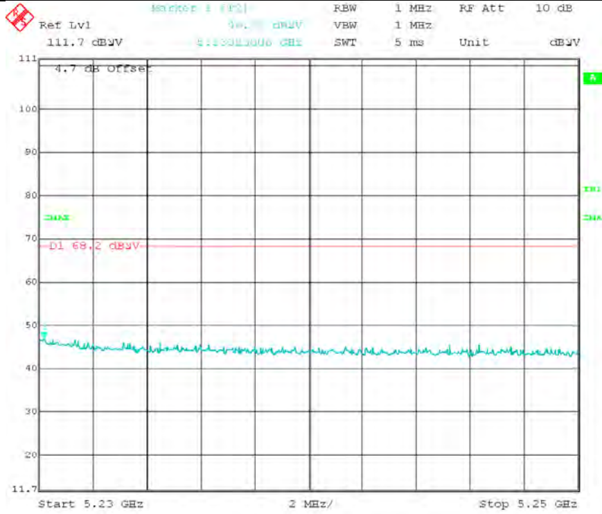
Low Channel (16MHz Mode 3)
