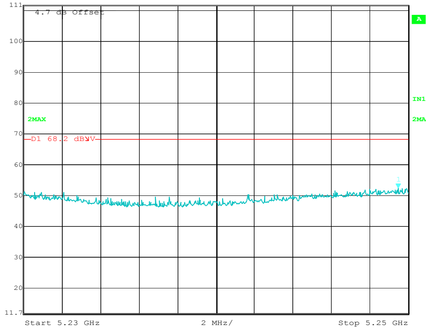
Low Channel (16MHz Mode 2)
