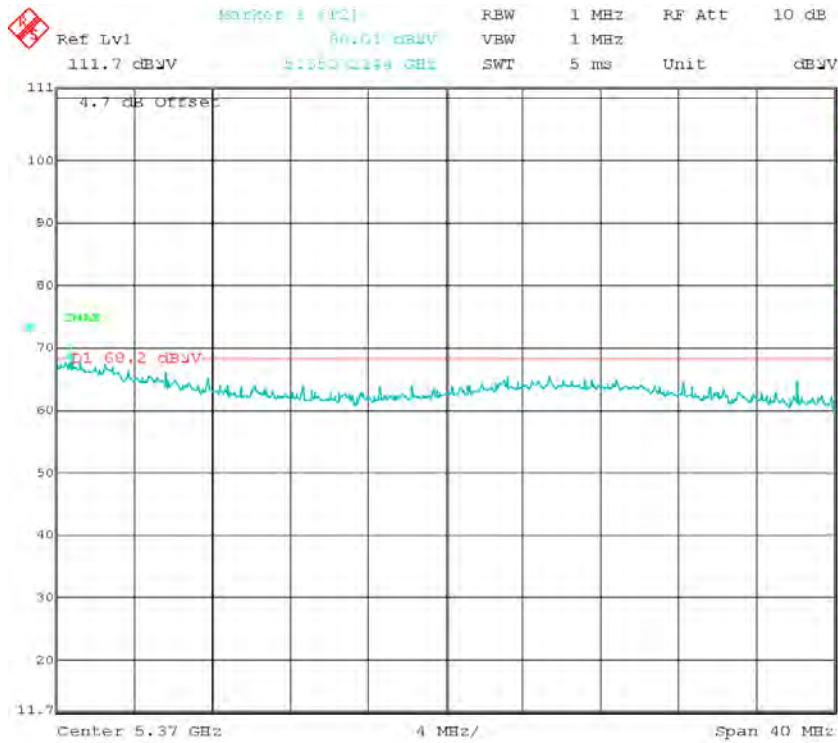
High Channel (32MHz Mode 1)
