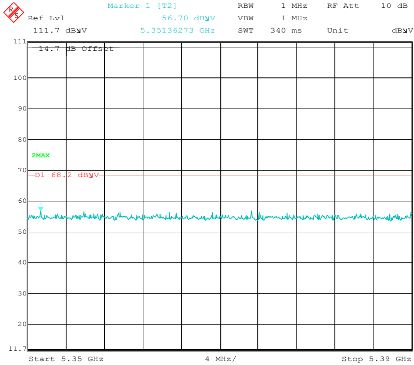
High Channel (32MHz Mode 2)
