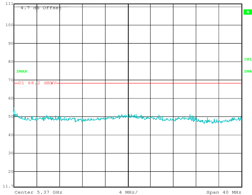
High Channel (32MHz Mode 1)
