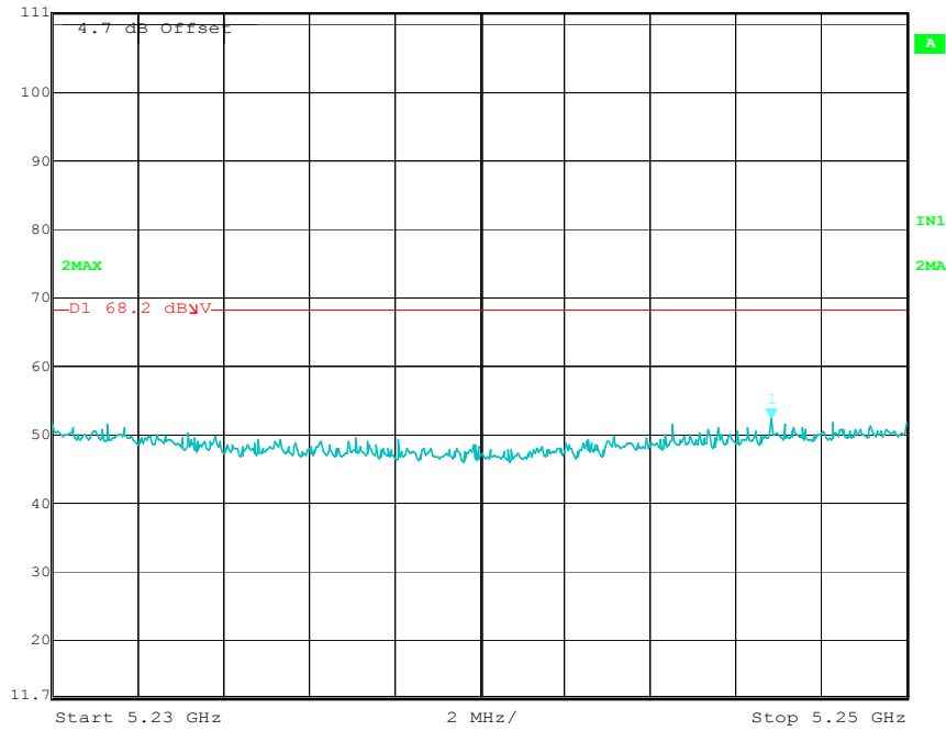
Low Channel (16MHz Mode 1)
