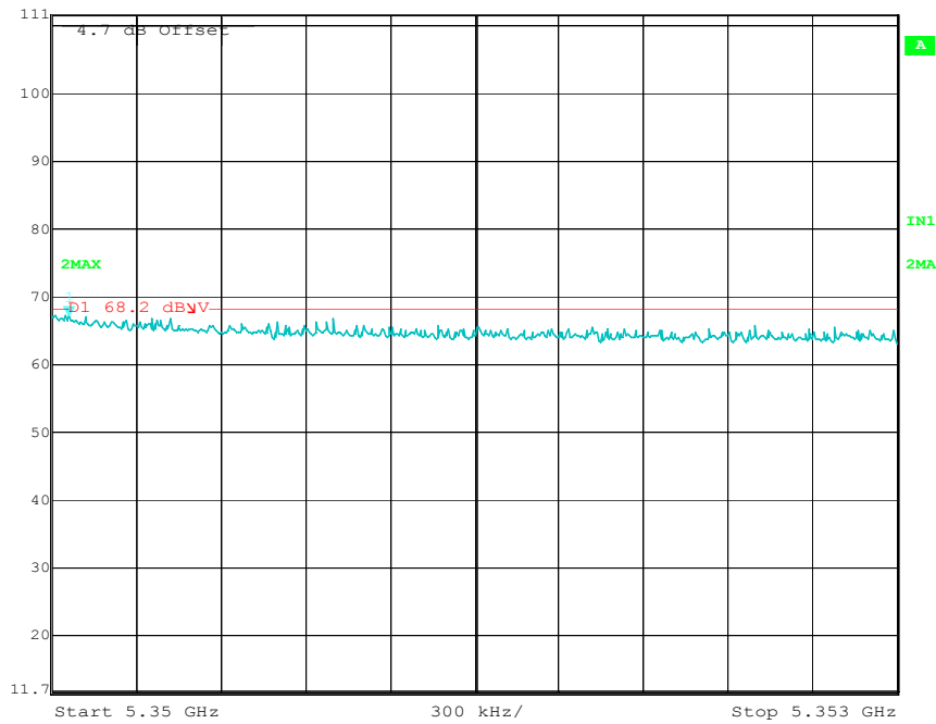
High Channel (8MHz Mode 3)
