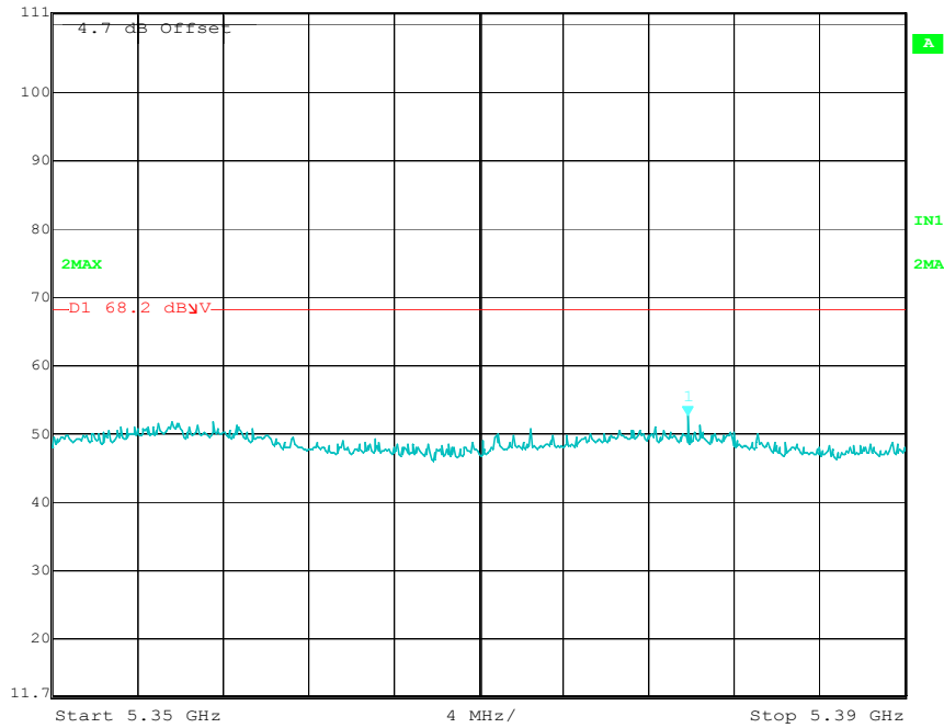
High Channel (32MHz Mode 2)
