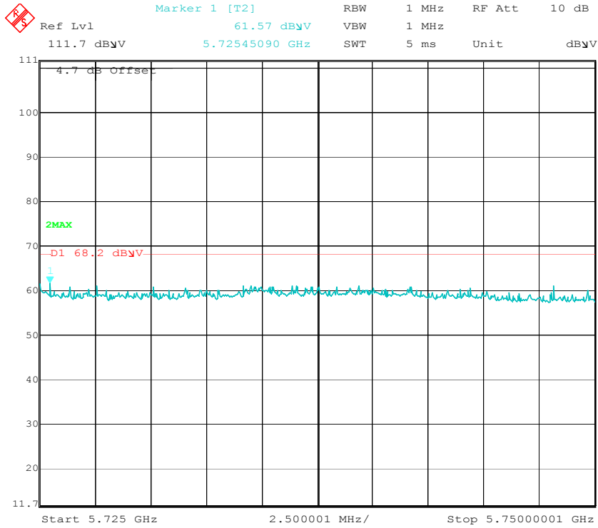
High Channel (16MHz Mode 2)
