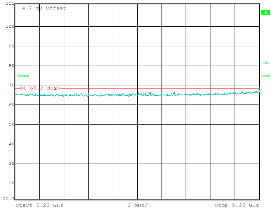
Low Channel (16MHz Mode 1)
