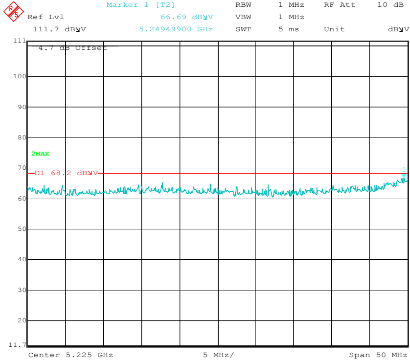
Low Channel (32MHz Mode 3)
