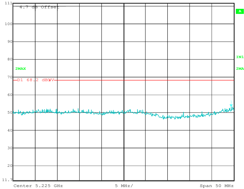
Low Channel (32MHz Mode 1)
