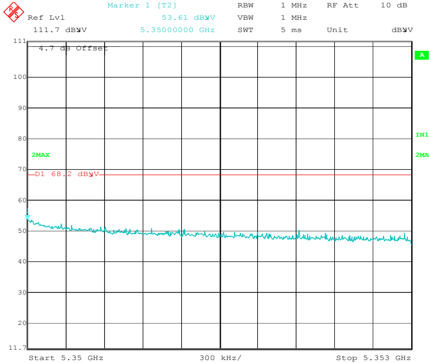
High Channel (16MHz Mode 1)
