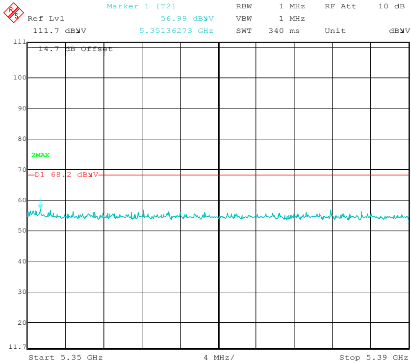
High Channel (32MHz Mode 3)
