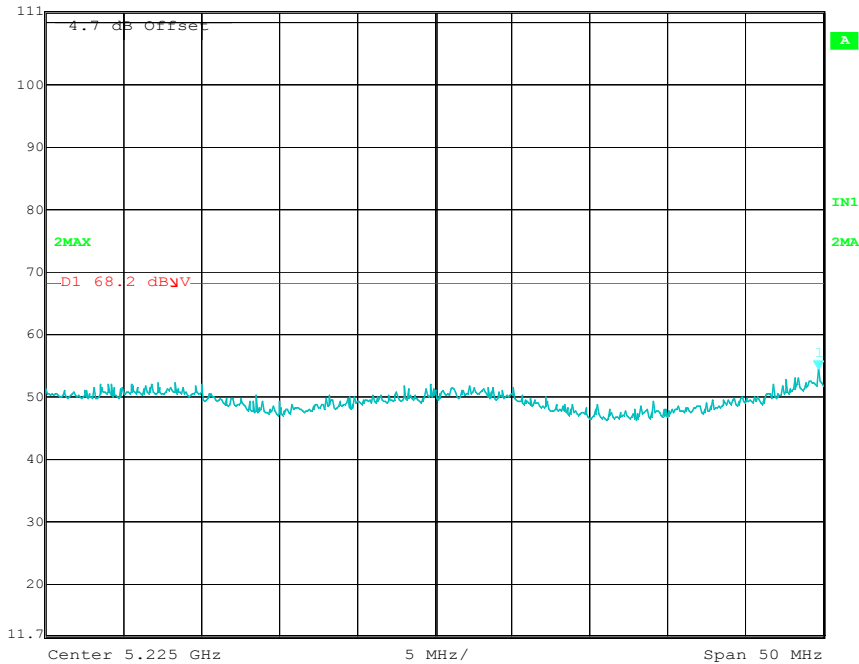
Low Channel (32MHz Mode 2)
