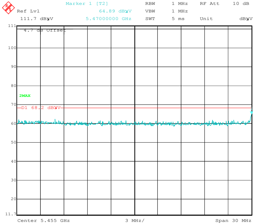
Low Channel (16MHz Mode 3)
