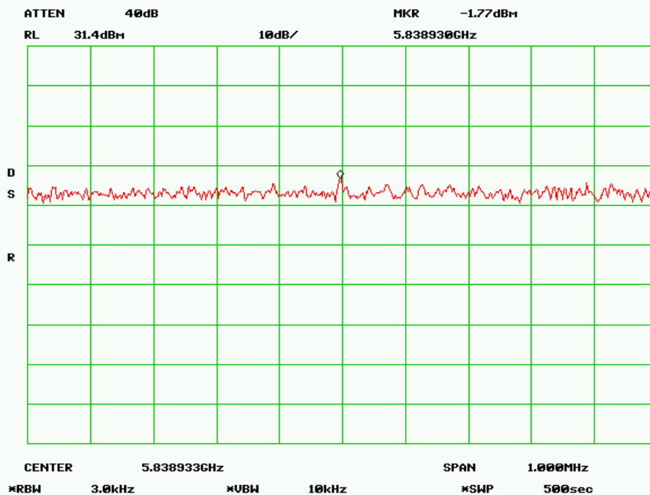
High Channel (16MHz Mode 3)
