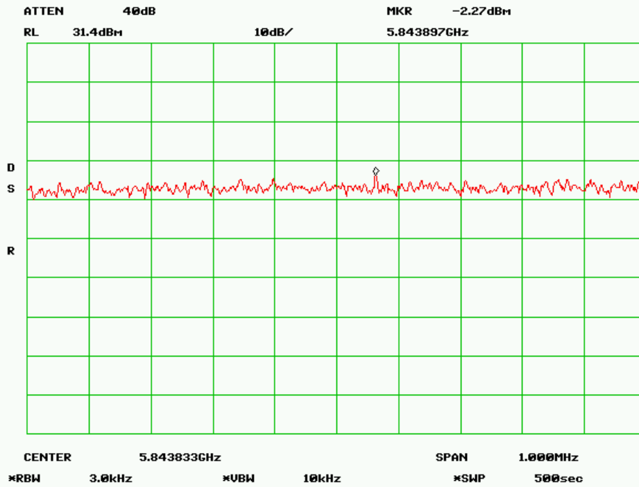
High Channel (16MHz Mode 2)
