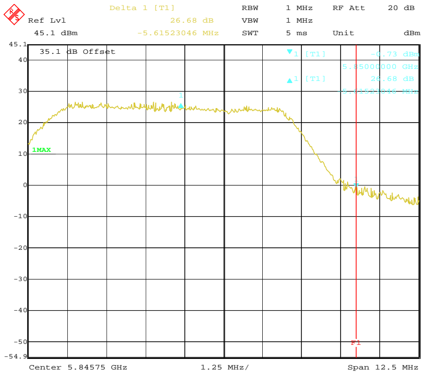
High Channel (8MHz Mode 3)
