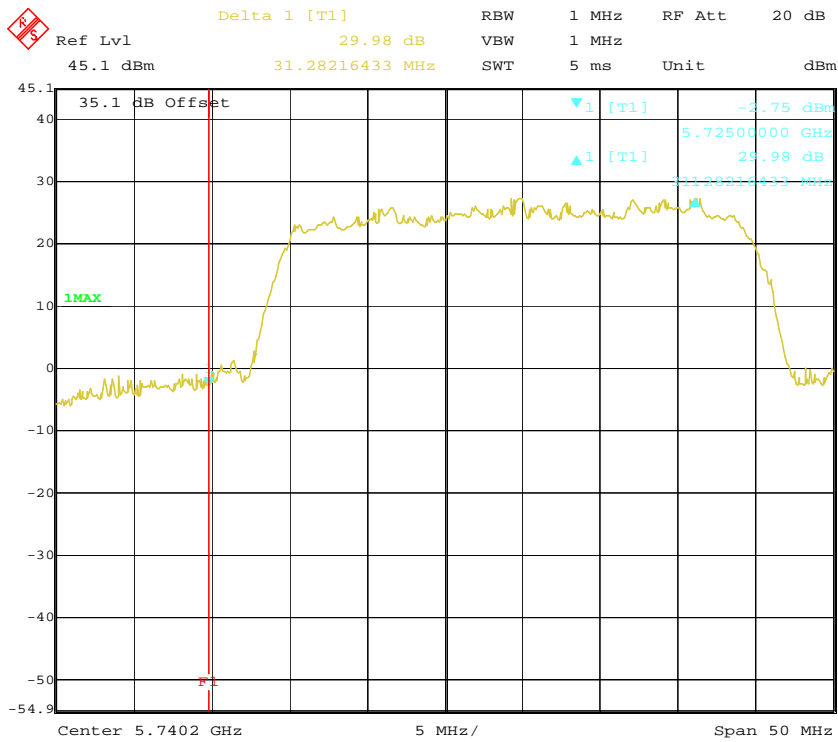
Low Channel (32MHz Mode 2)
