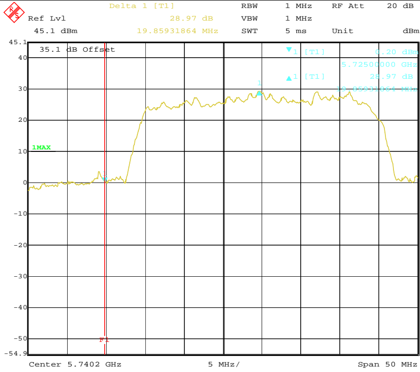
Low Channel (32MHz Mode 1)
