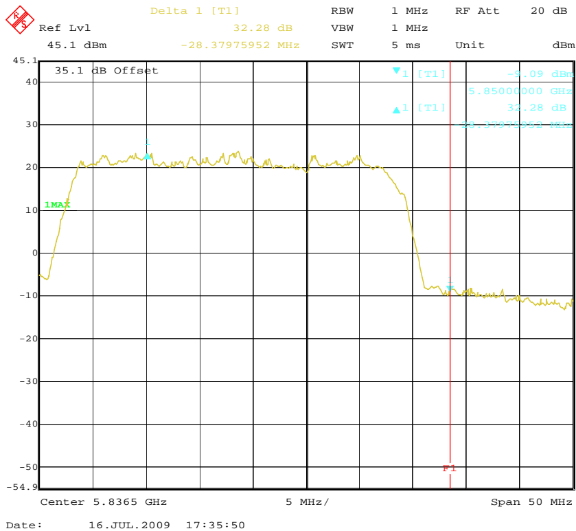
High Channel (32MHz Mode 3)
