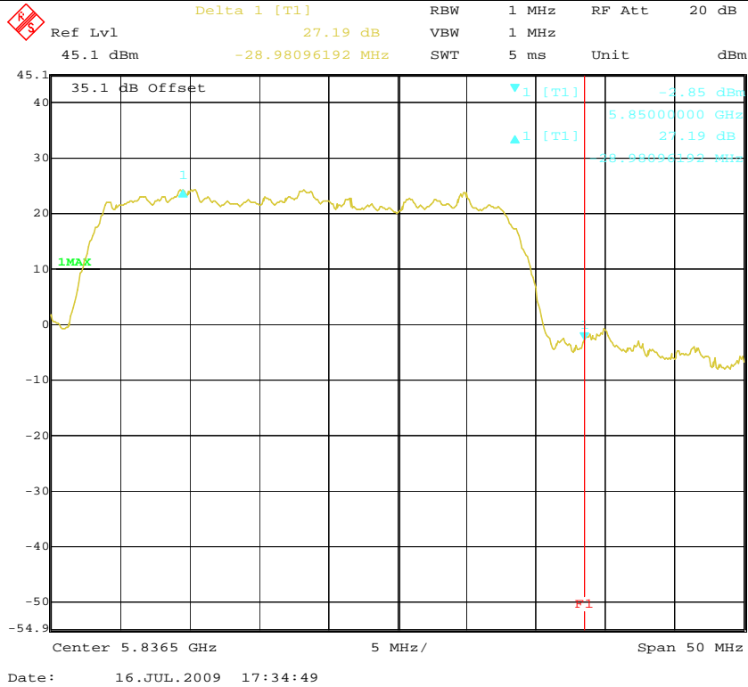
High Channel (32MHz Mode 2)
