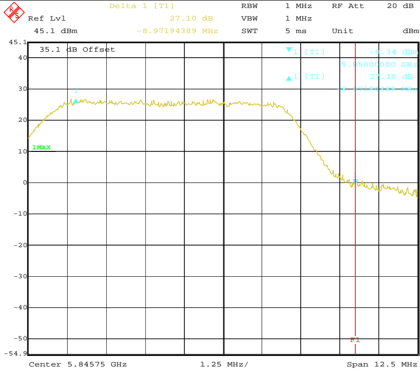
High Channel (8MHz Mode 2)
