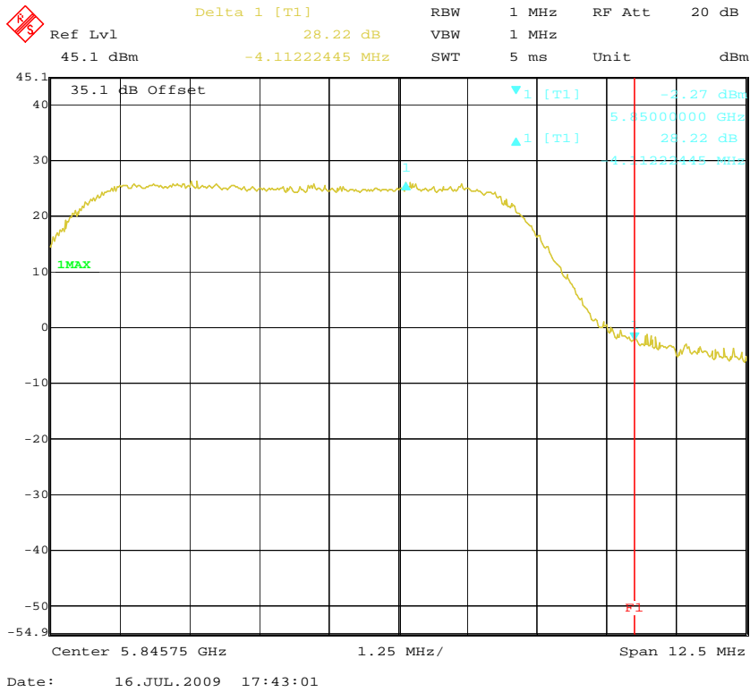
High Channel (8MHz Mode 1)
