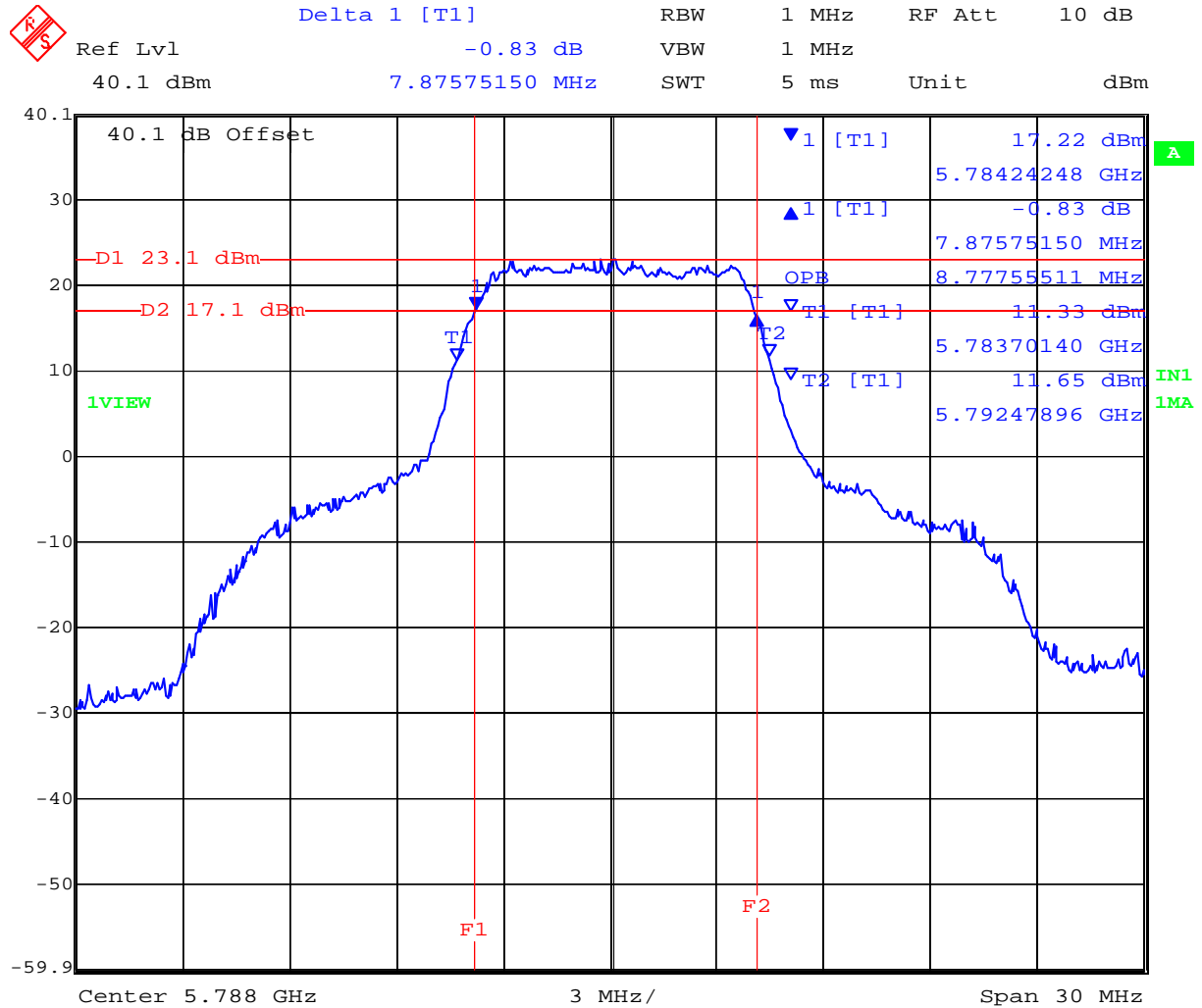
Plot A02 5,788 MHz 7.5 MHz 64QAM 6 dB & 99% Bandwidth
