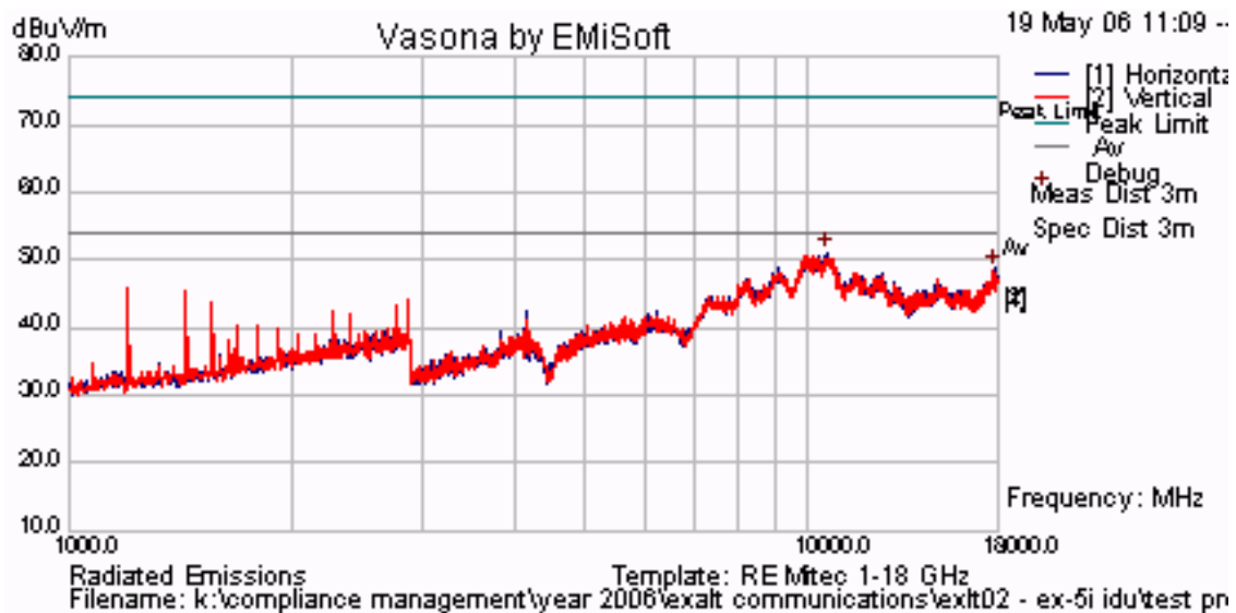
5,788 MHz Radiated Emissions for 37.9 dBi Antenna 7.5 MHz Bandwidth QPSK
