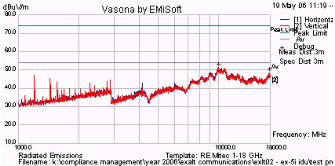
5,788 MHz Radiated Emissions for 37.9 dBi Antenna 15 MHz Bandwidth QPSK
