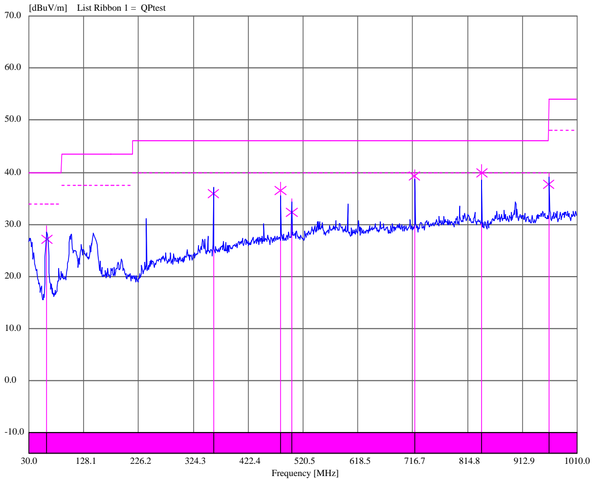
Plot 71 Radiated Spurious Emissions 30 MHz to 1 GHz
