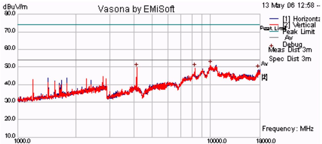
5,788 MHz Radiated Emissions for 28 dBi Antenna 7.5 MHz Bandwidth QPSK
