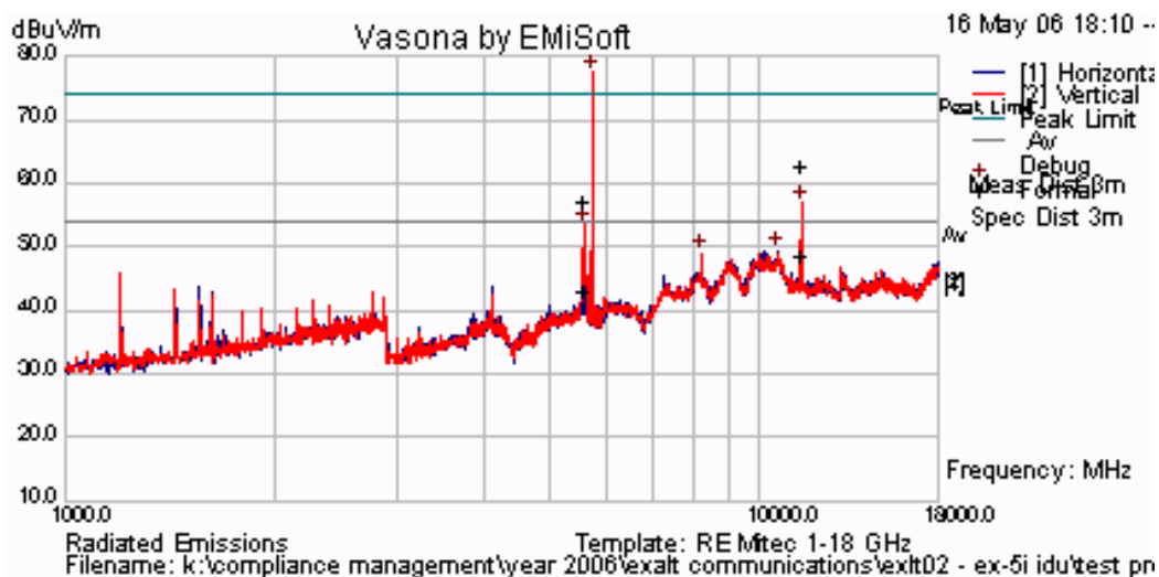
5,731 MHz Radiated Emissions for 37.9 dBi Antenna 7.5 MHz Bandwidth QPSK
