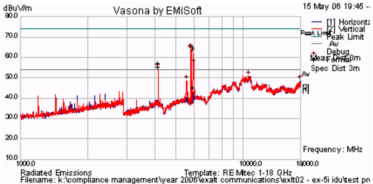
5,813 MHz Radiated Emissions for 28 dBi Antenna 60 MHz Bandwidth 16QAM
