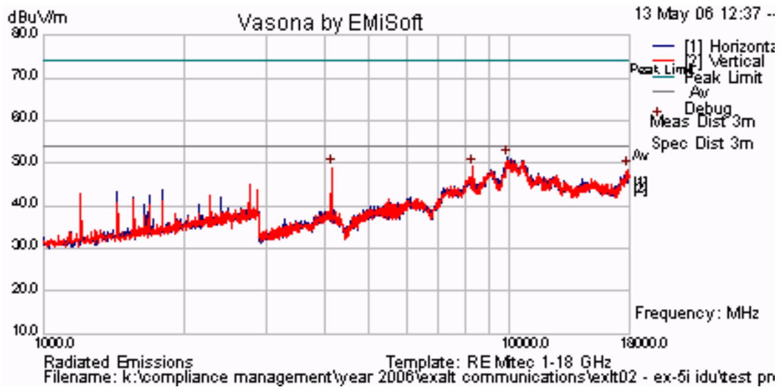
5,788 MHz Radiated Emissions for 28 dBi Antenna 30 MHz Bandwidth QPSK
