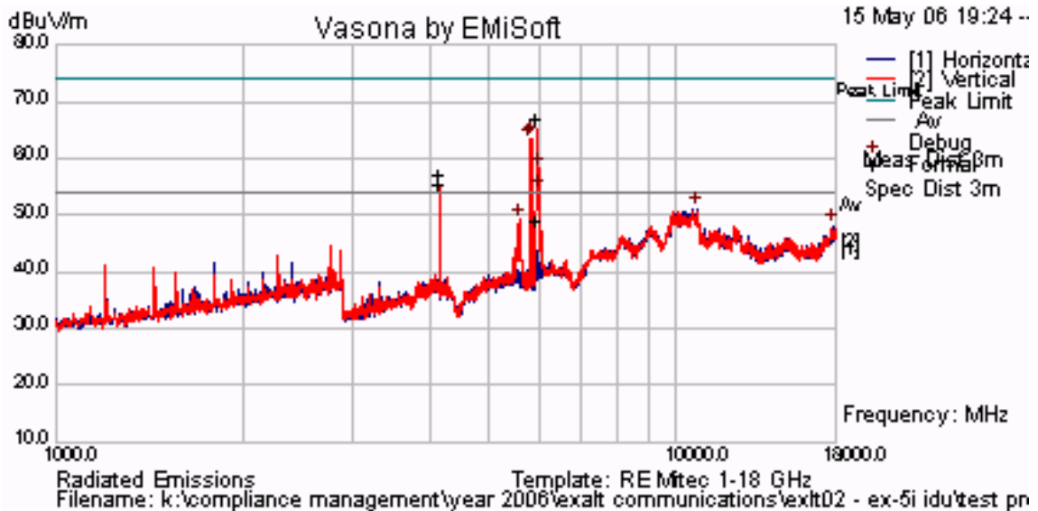
5,813 MHz Radiated Emissions for 28 dBi Antenna 60 MHz Bandwidth 64QAM
