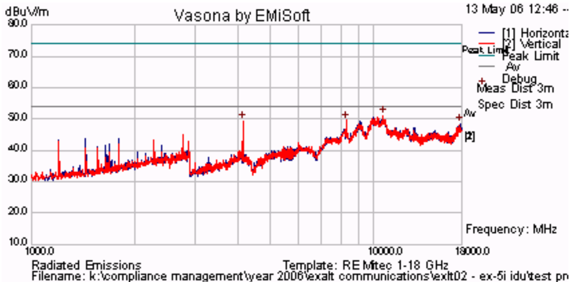
5,788 MHz Radiated Emissions for 28 dBi Antenna 60 MHz Bandwidth QPSK
