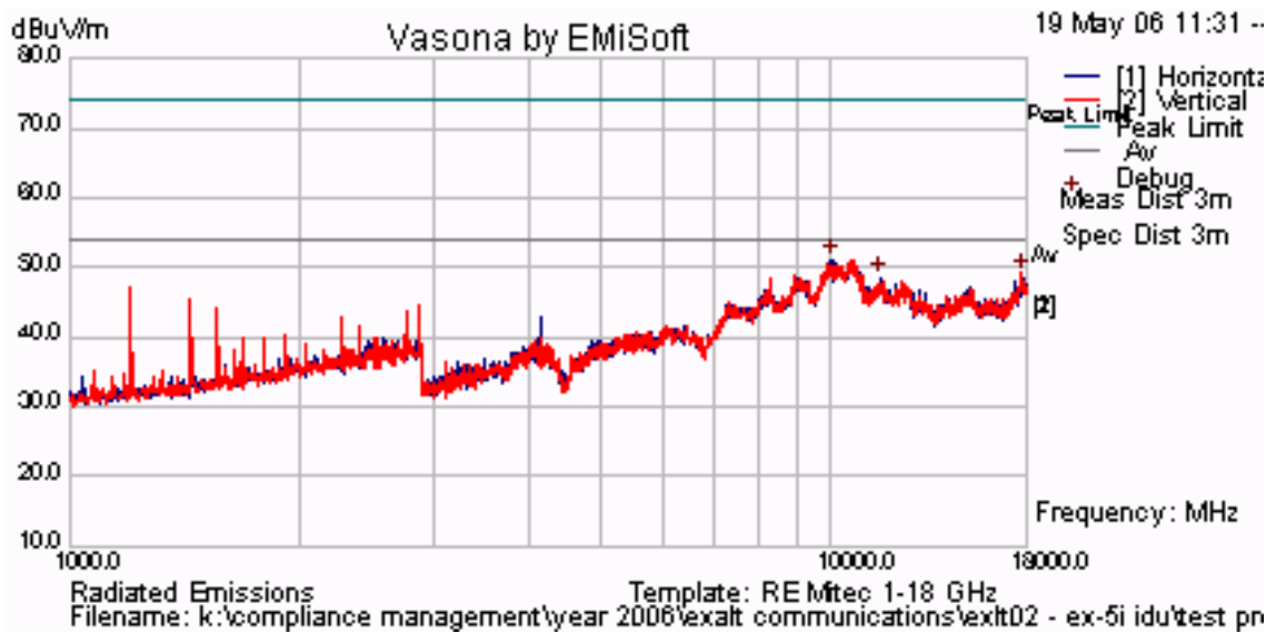
5,788 MHz Radiated Emissions for 37.9 dBi Antenna 30 MHz Bandwidth QPSK
