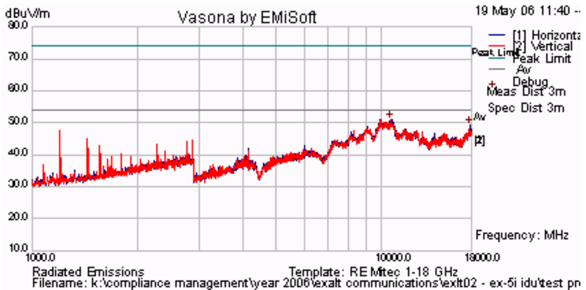
5,788 MHz Radiated Emissions for 37.9 dBi Antenna 60 MHz Bandwidth QPSK
