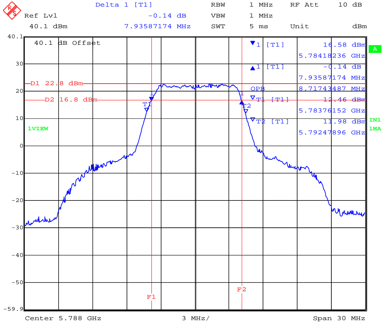
Plot A01 5,788 MHz 7.5 MHz 16QAM 6 dB & 99% Bandwidth
