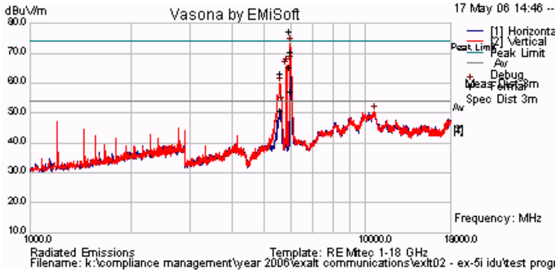
5,813 MHz Radiated Emissions for 37.9 dBi Antenna 60 MHz Bandwidth QPSK
