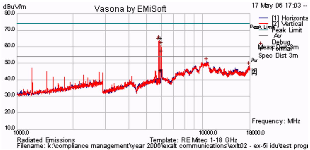
5,813 MHz Radiated Emissions for 37.9 dBi Antenna 60 MHz Bandwidth 64QAM
