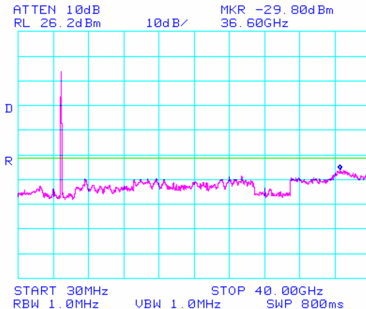
Spurious Emissions QPSK 20 MHz BW 4965 MHz 30 MHz – 40 GHz: Limit -25 dBm
