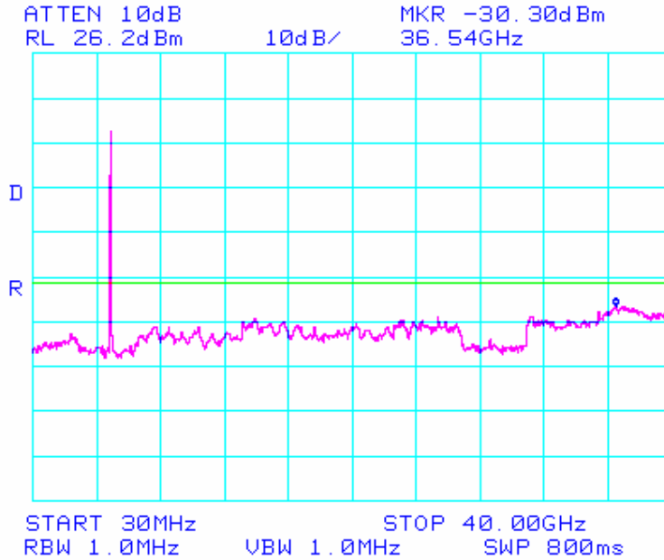
Spurious Emissions QPSK 20 MHz BW 4950 MHz 30 MHz – 40 GHz: Limit -25 dBm
