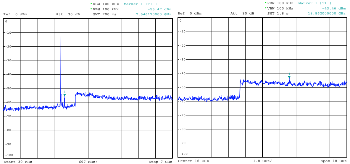
Figure 5. Plot of the Spurious Emission (Conducted)
