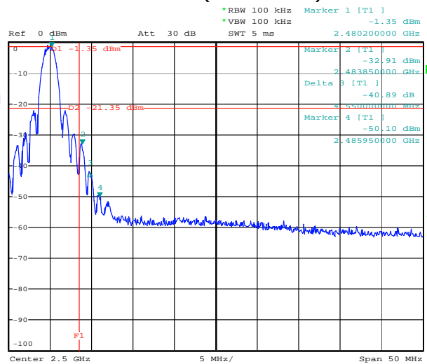
Figure 4. Plot of the Bandedge Compliance (Conducted)
