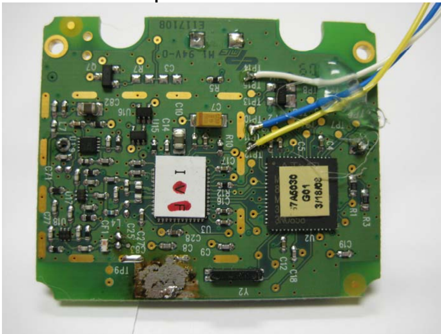
Close Up View #2 of RF Section
