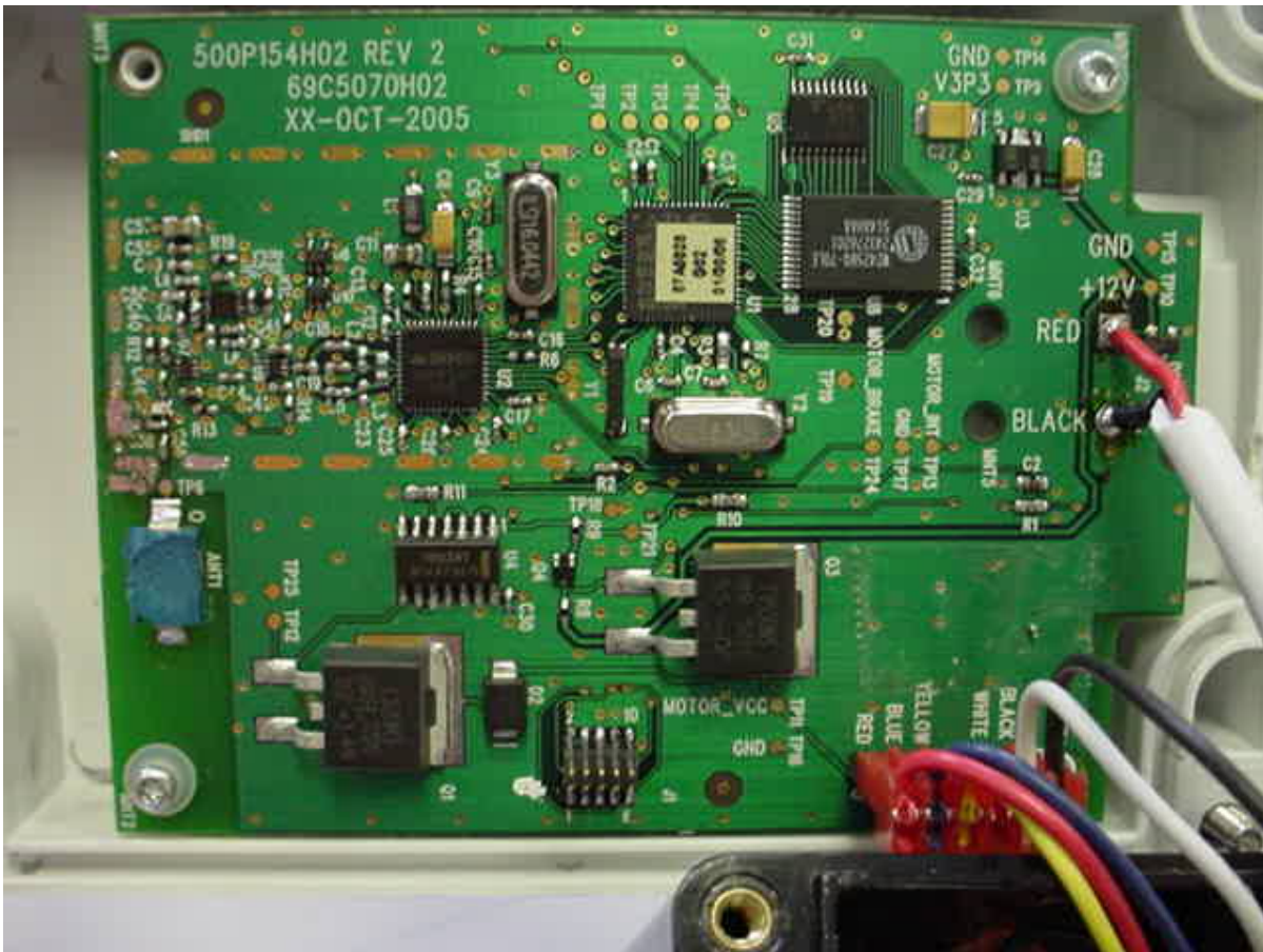
Photo Two – Internal Front Side of RF Board
