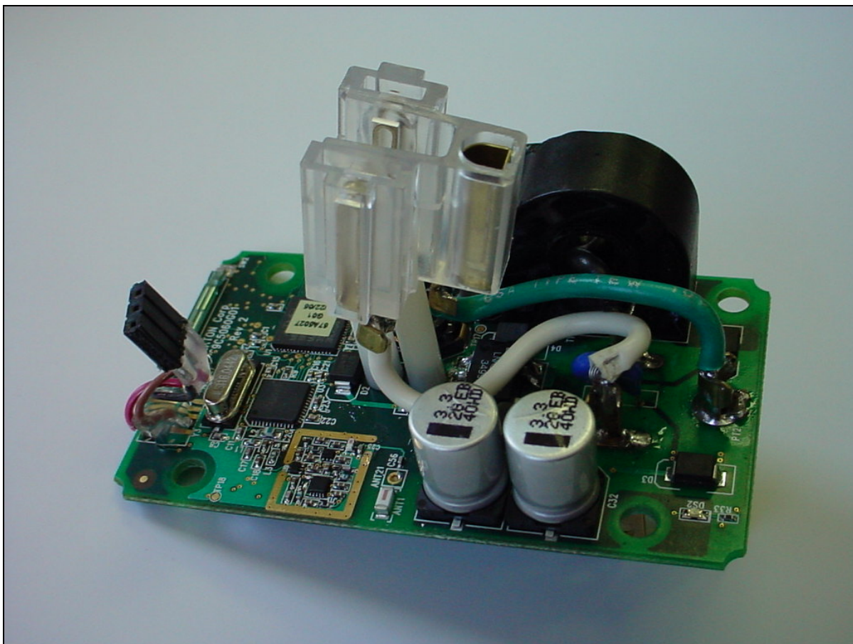
Photo Two – Internal Open for Inspection-complete PCB
