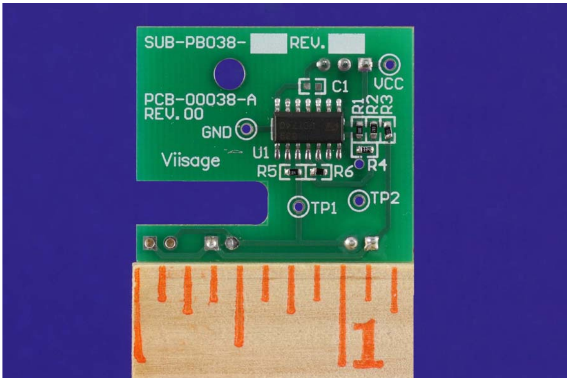
Document Detect Board – Rear:
