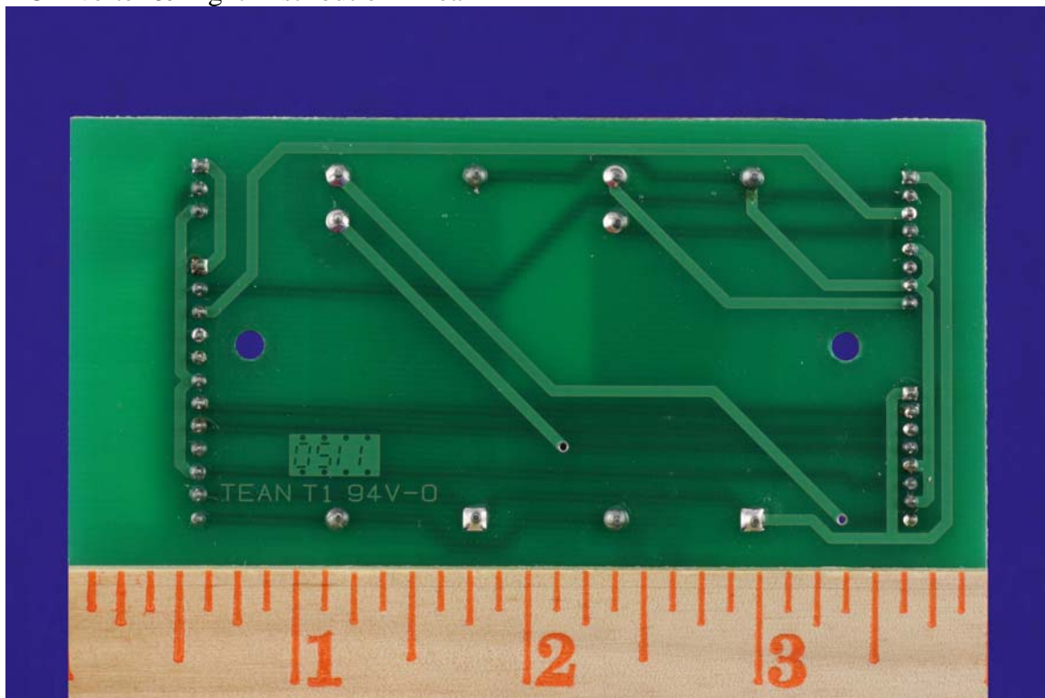
DC Inverter & Light Distribution - Rear
