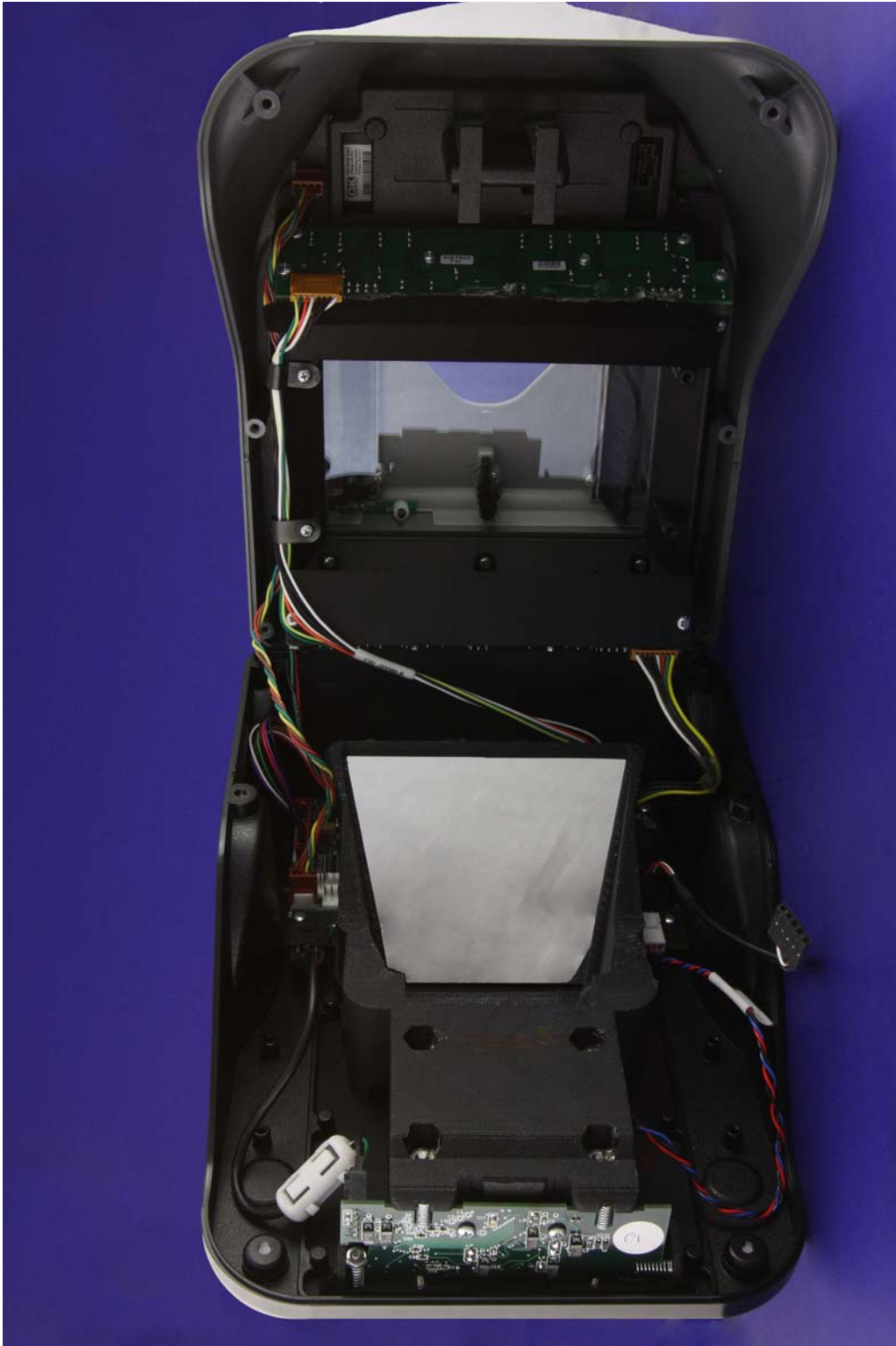
Internal Photos – Viisage BS5000-SC
