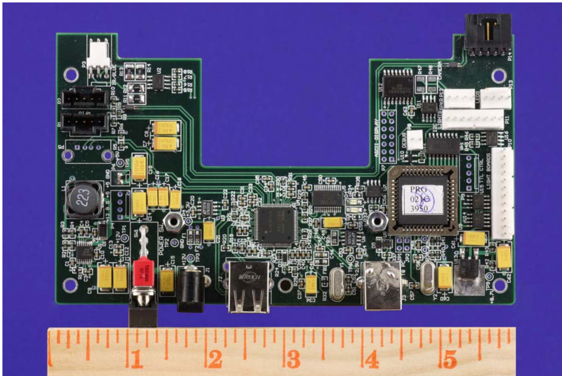
Main Control Board – Front:
