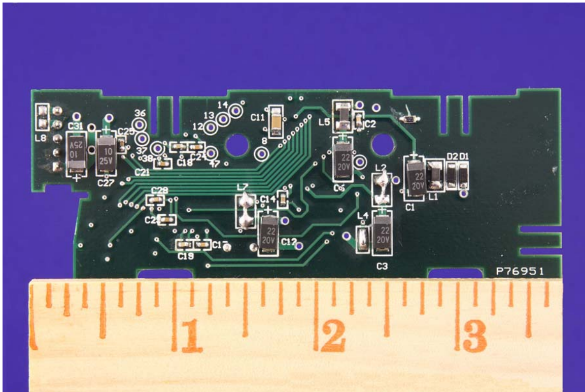
Camera Board – Rear:
