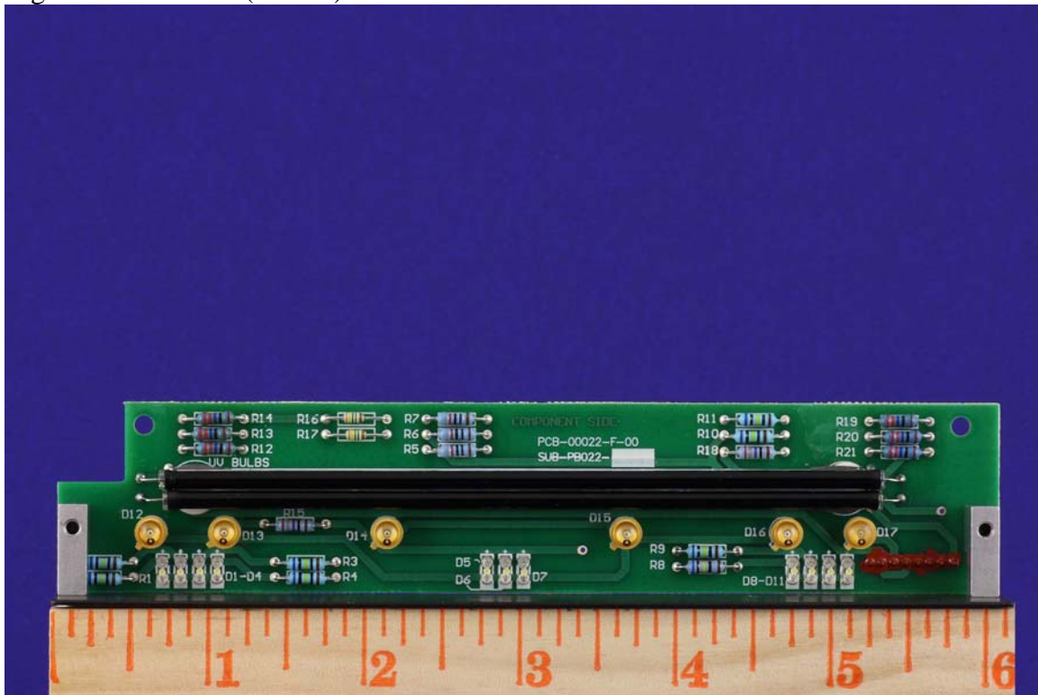
Light Board – Rear (2 Used):
