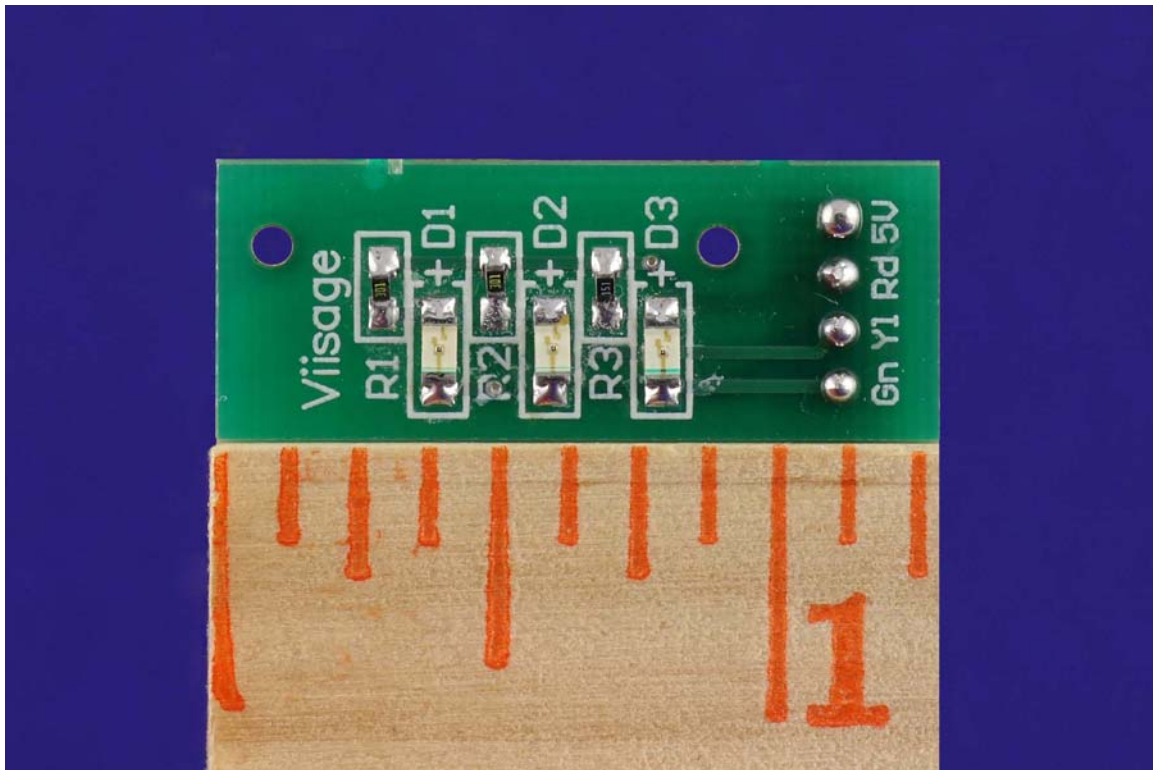
Status LED Board – Front:
