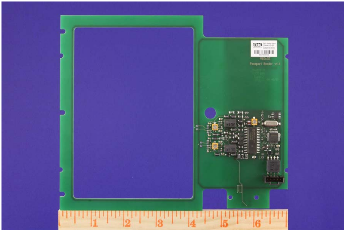
Antenna Board – Front:
