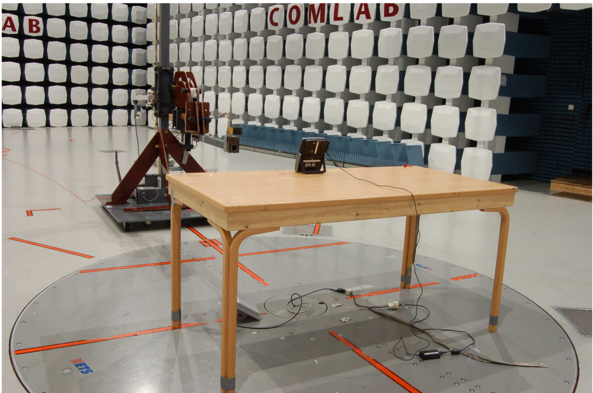
Radiated emissions 12 GHz – 18 GHz
