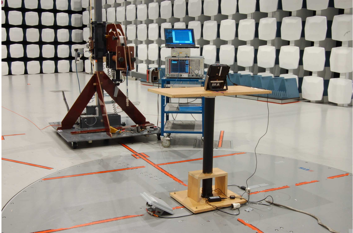
Radiated emissions 18 – 20 GHz
