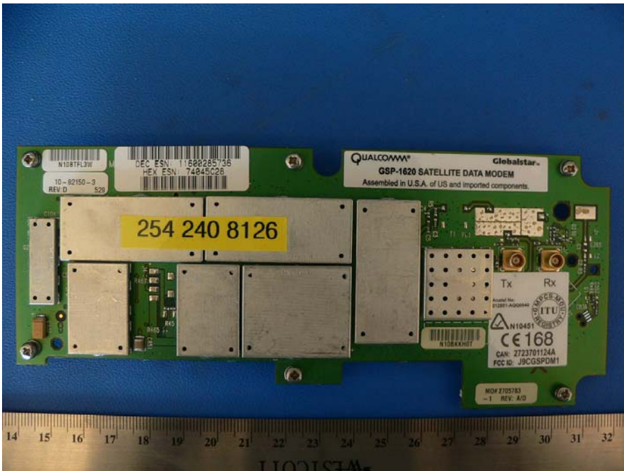
Data modem Component side View
