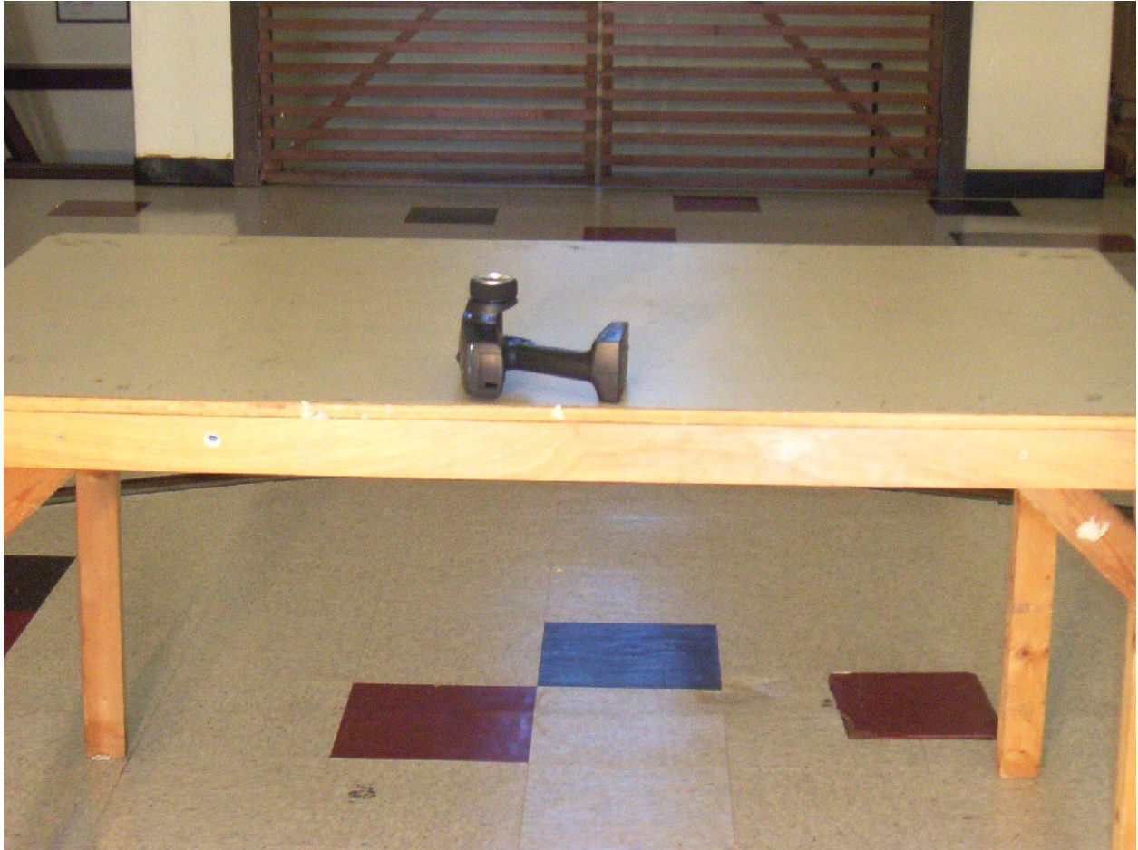
Photo 3: Radiated Emission Test Setup – EUT Standalone, Side Position View 1
