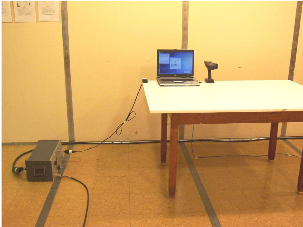
Photo 3: Conducted Emission Test Setup, USB Interface mode with Ethernet I/O at PC, Front View
