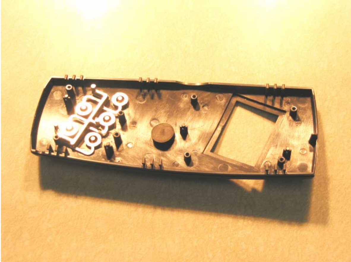
Photo 5: Internal View of Top Cover
