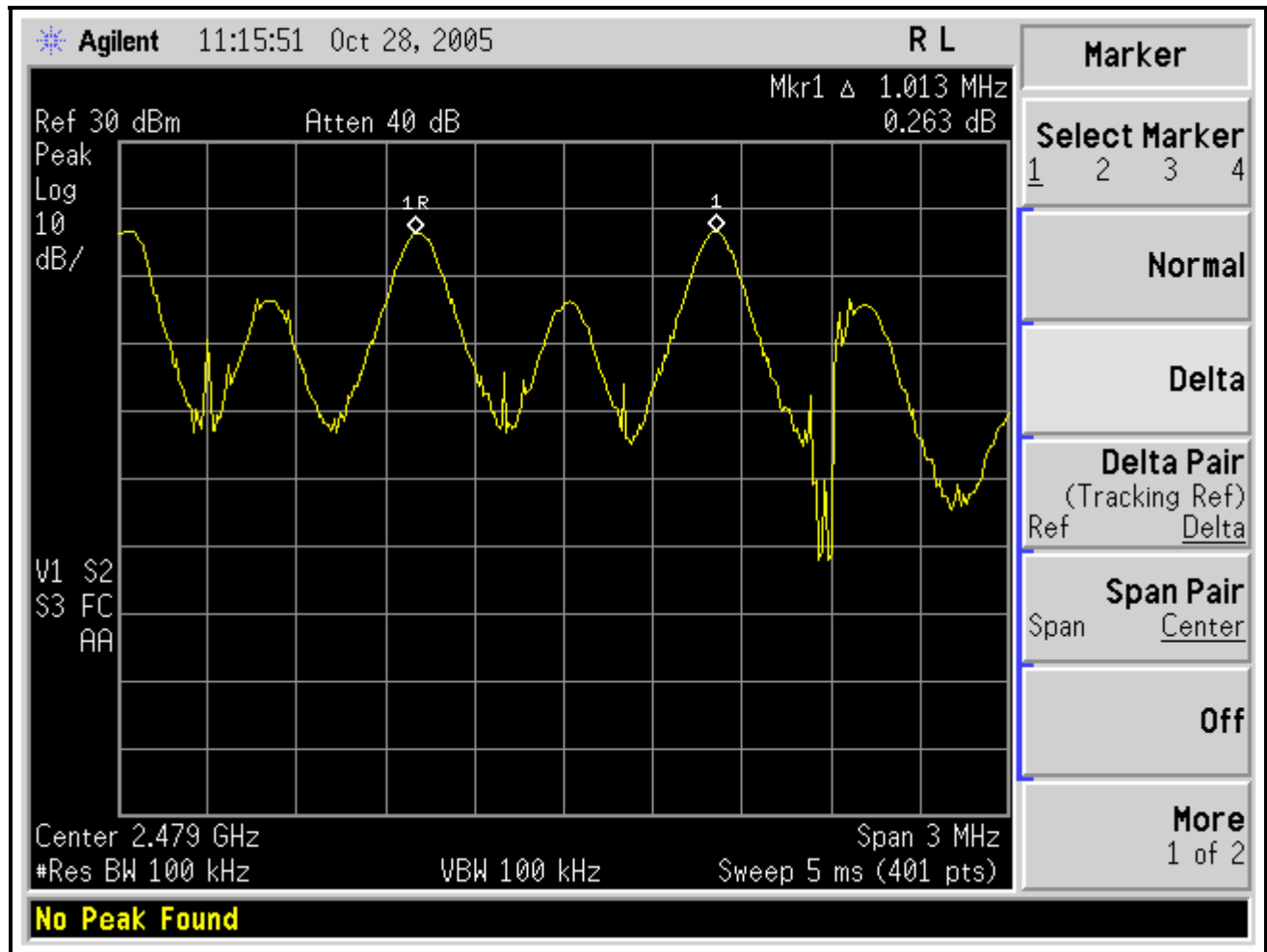
Plot 6. Channel Separation between Channel 77 and Channel 78
