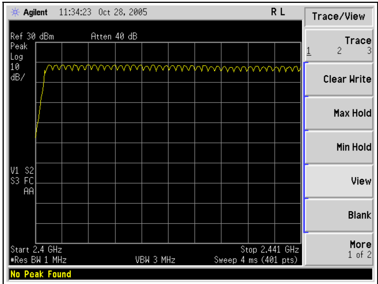
Plot 7. Number of Channels – Part 1
