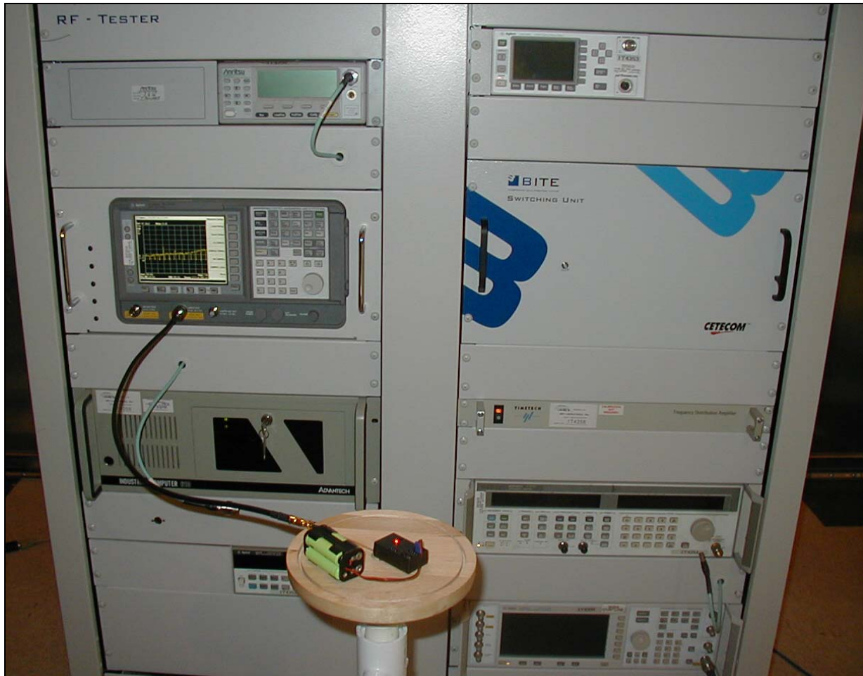
Photograph 3. Bandwidth and Channel Separation Test Setup
