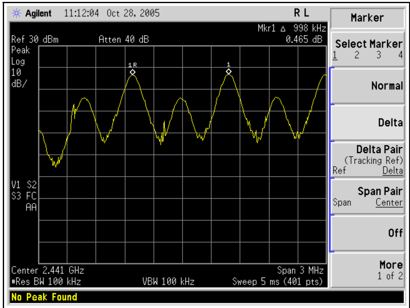
Plot 5. Channel Separation between Channel 38 and Channel 39
