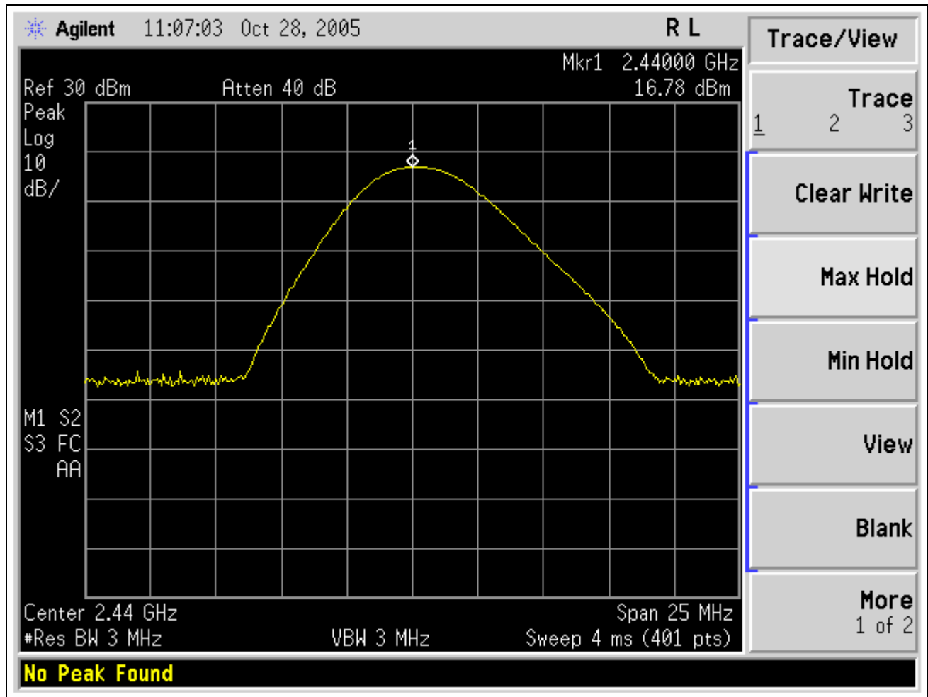
Plot 12. Peak Power Output Test Results – Channel 38
