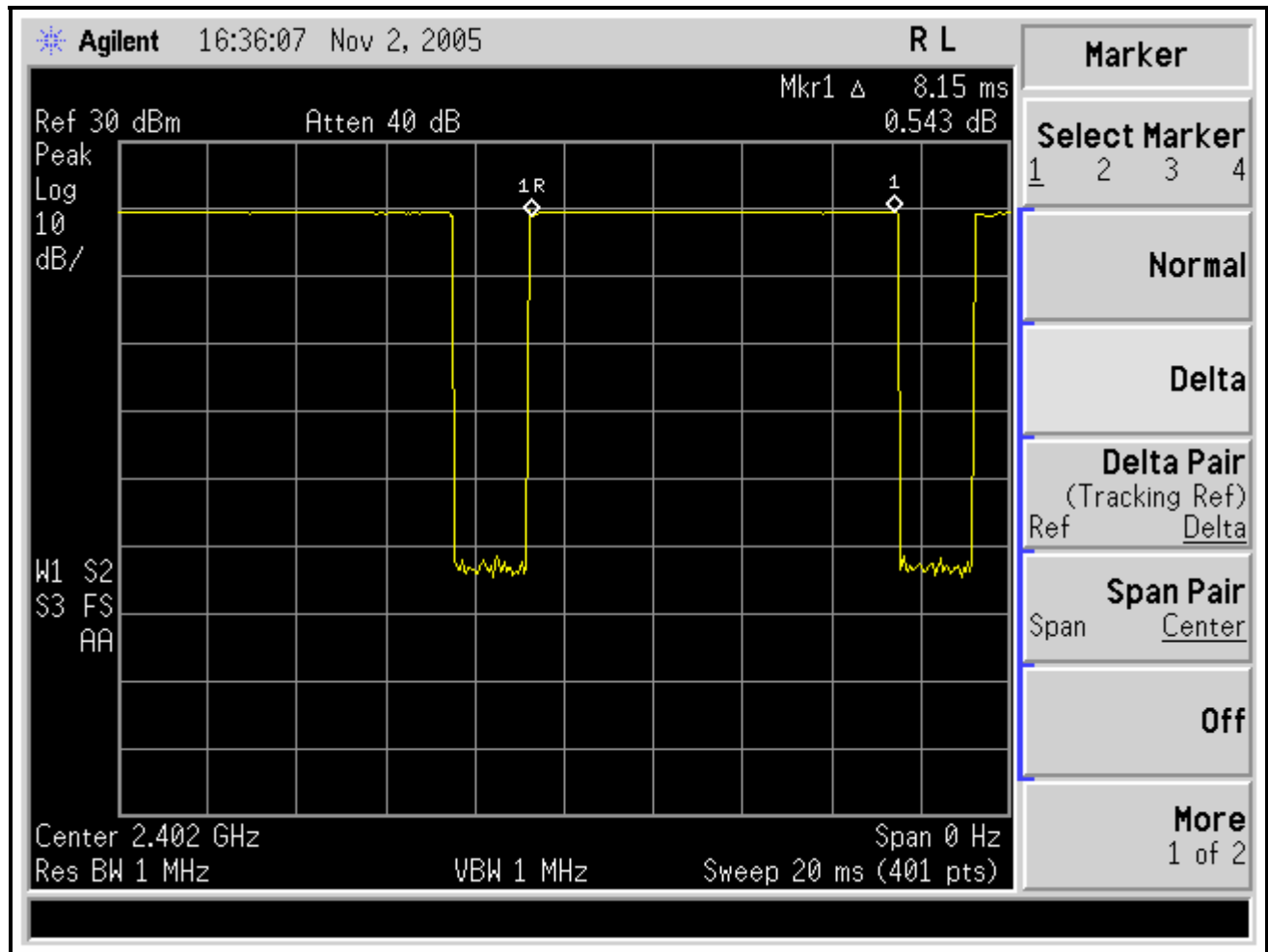
Plot 9. Dwell Time of an Individual Channel
