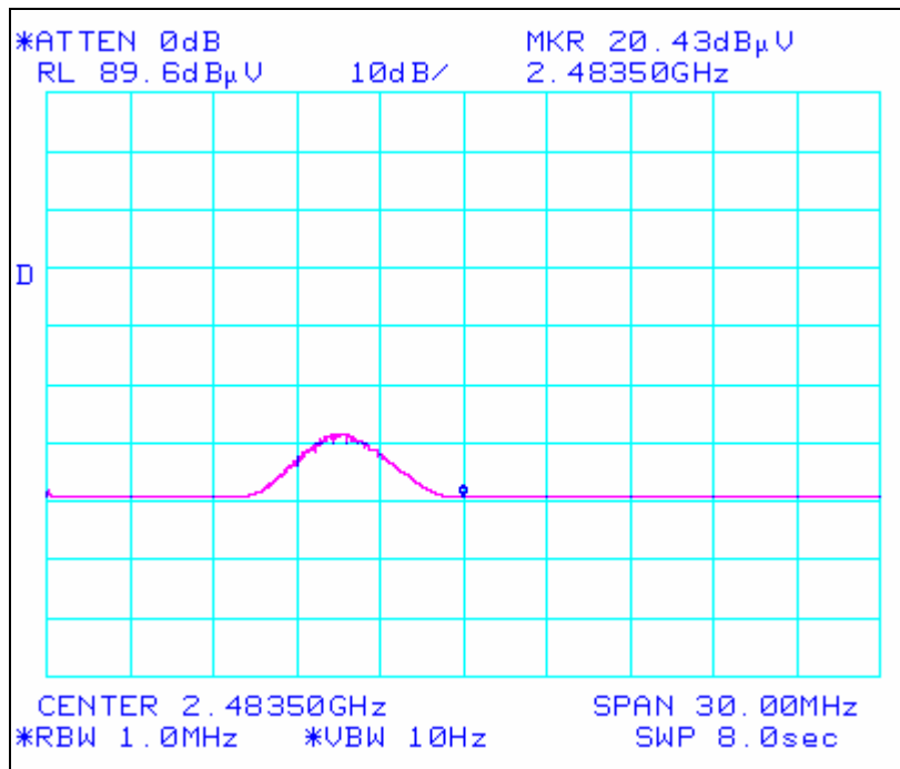
Plot 18. Band Edge Test Results, Channel 78 - Average
