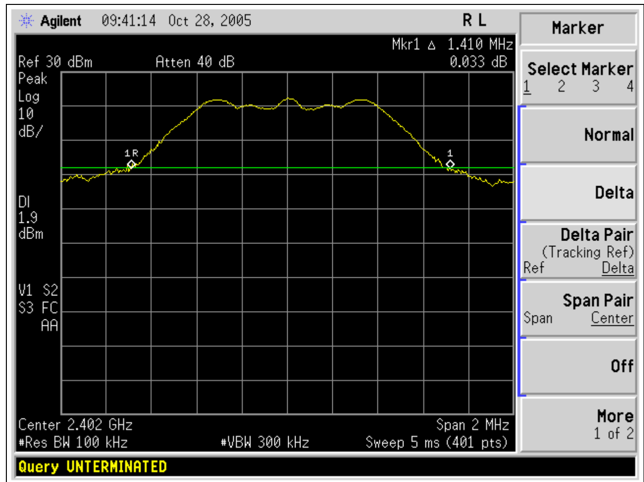
Plot 1. Occupied Bandwidth; Test Results, Channel 1
