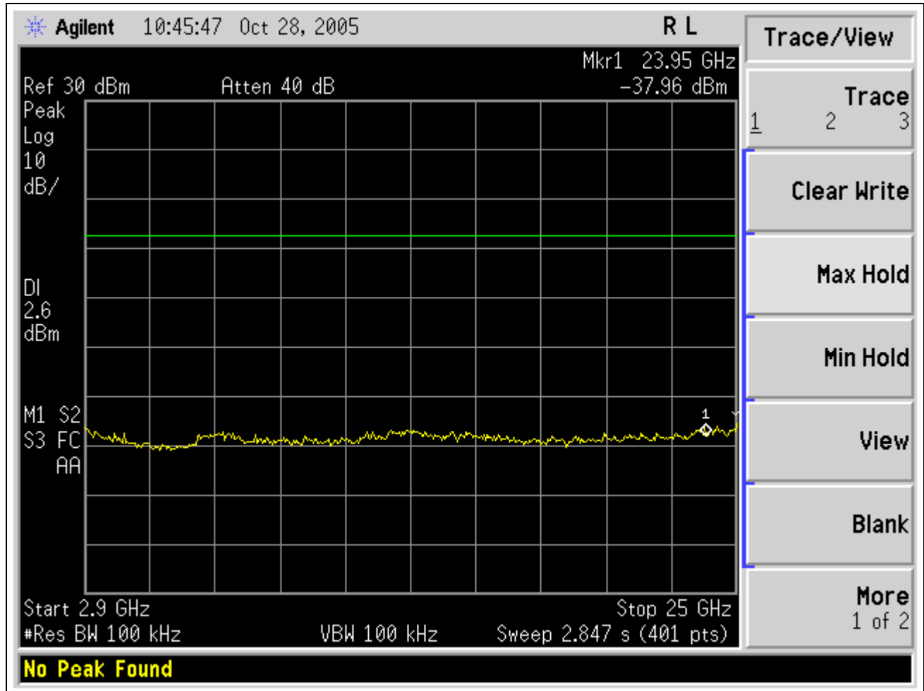
Plot 16. Spurious Conducted Emission Test Plot – 2.9 GHz to 25 GHz
