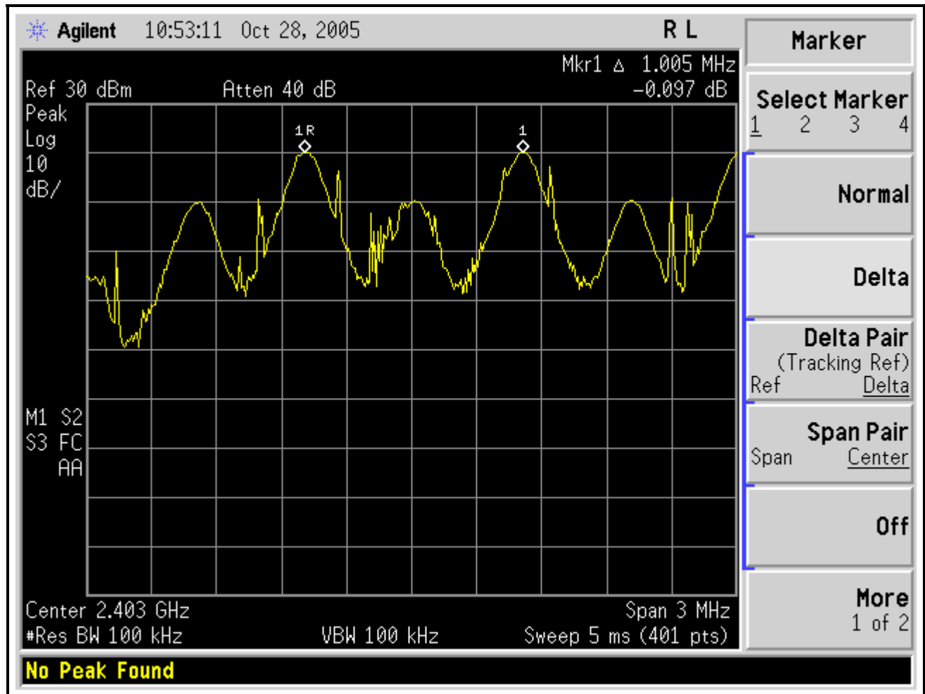
Plot 4. Channel Separation between Channel 1 and Channel 2
