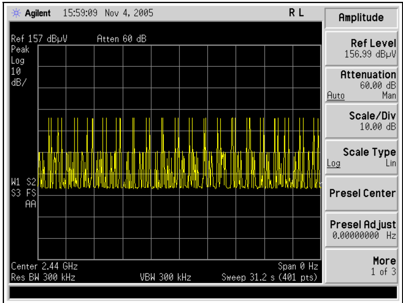
Plot 10. Number of Times a Channel is Repeated in a .31.2 second Period
