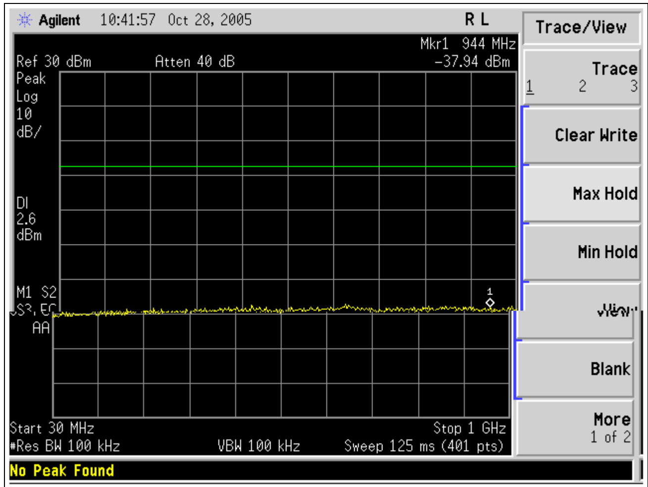
Plot 14. Spurious Conducted Emission Test Plot – 30 MHz to 1 GHz
