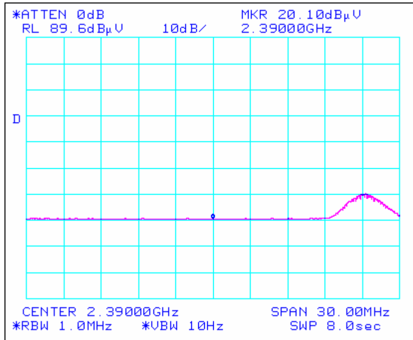
Plot 17. Band Edge Test Results, Channel 1 - Average
