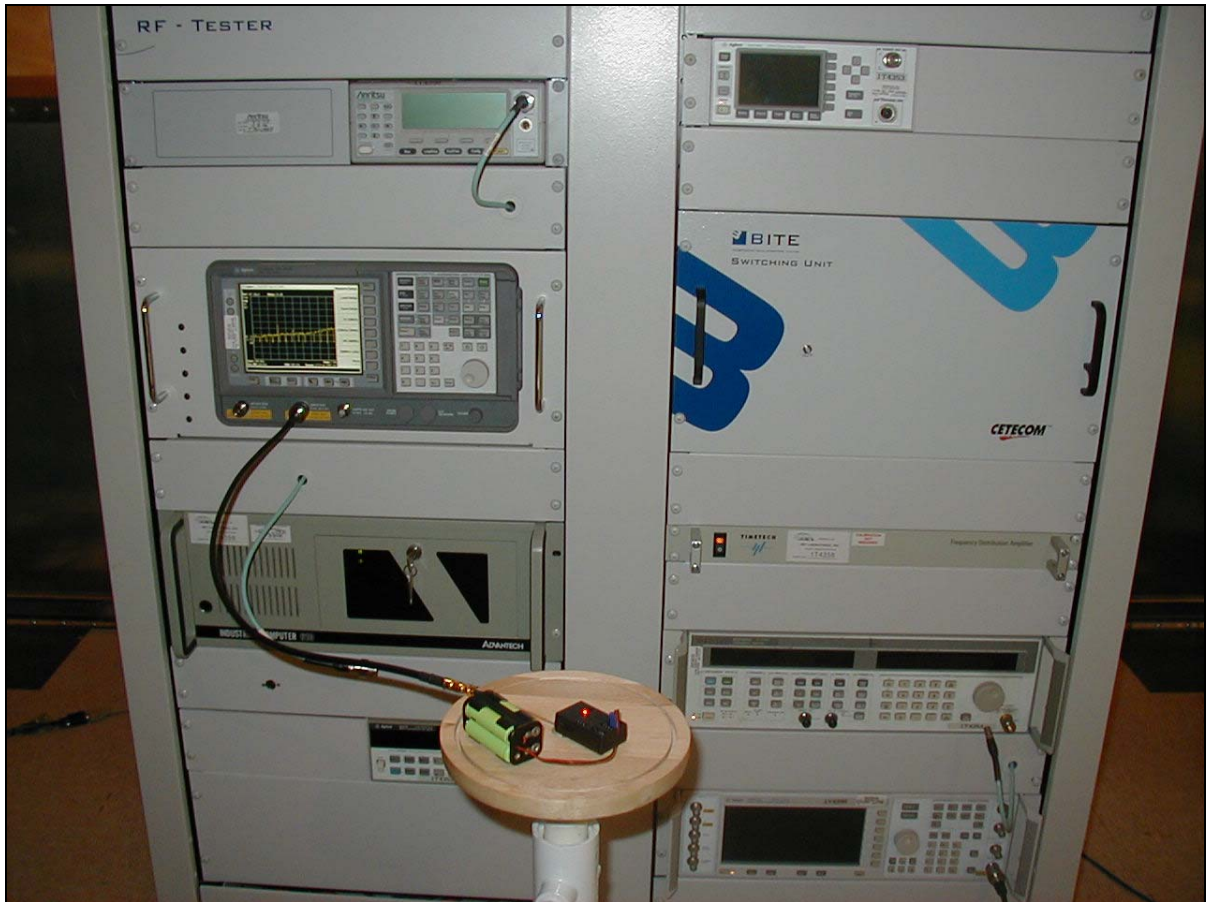
Photograph 4. Number of Channels and Time of Occupancy Test Setup
