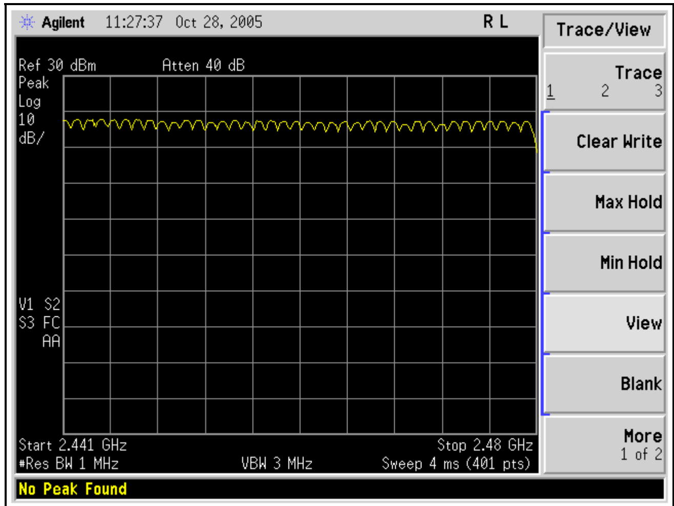
Plot 8. Number of Channels – Part 2
