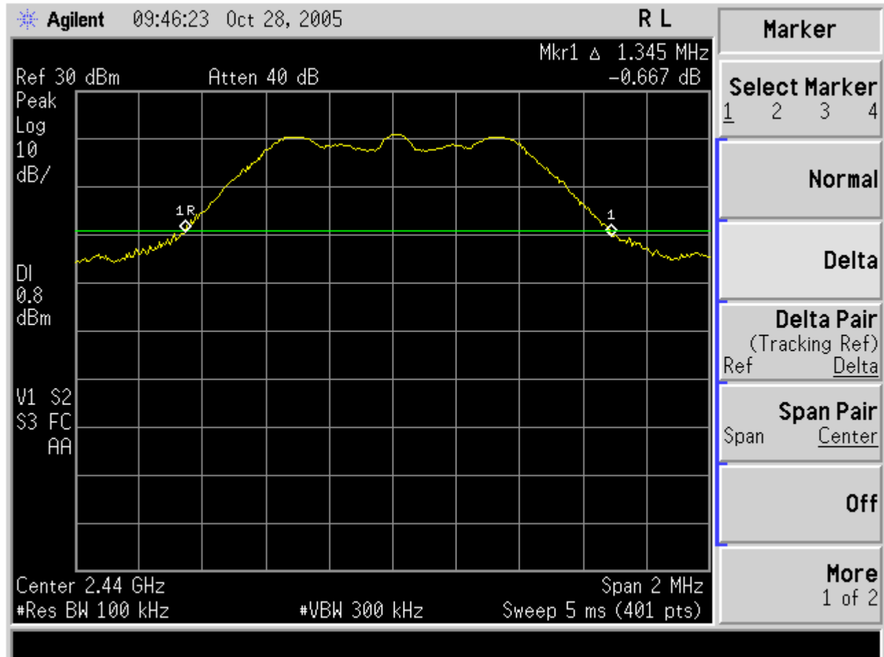
Plot 2. Occupied Bandwidth; Test Results, Channel 38
