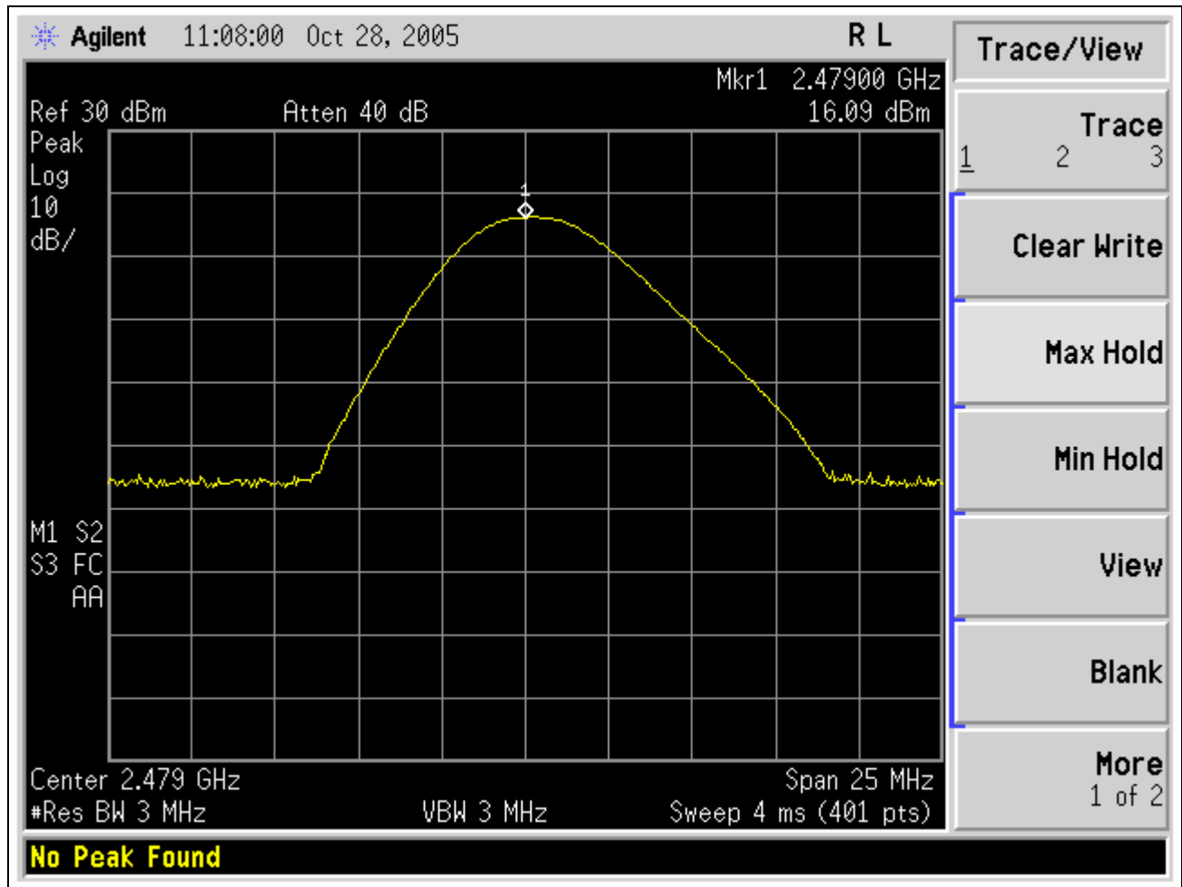
Plot 13. Peak Power Output Test Results – Channel 78
