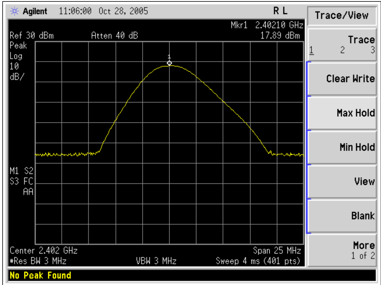
Plot 11. Peak Power Output Test Results – Channel 1
