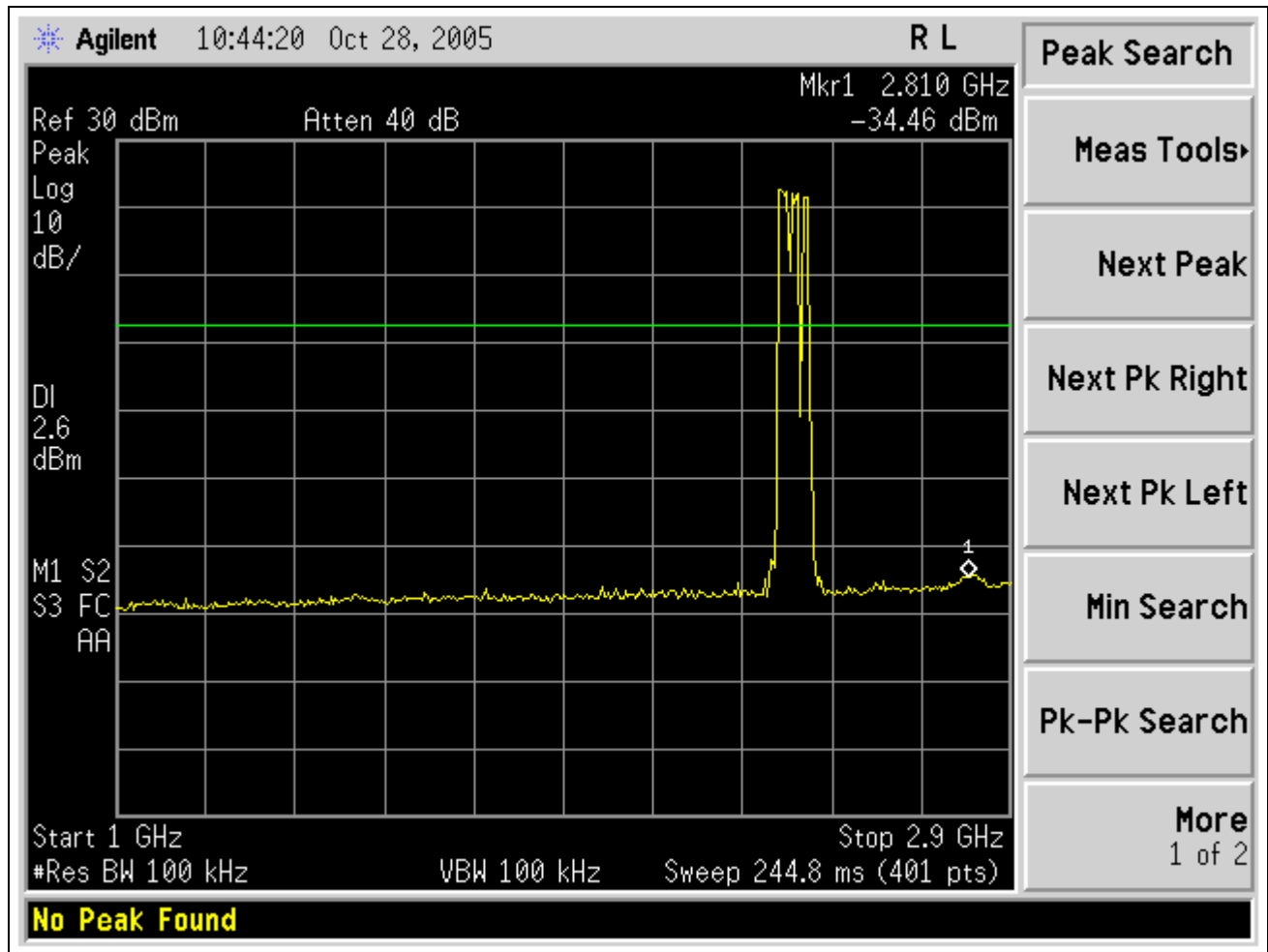
Plot 15. Spurious Conducted Emission Test Plot – 1 GHz to 2.9 GHz
