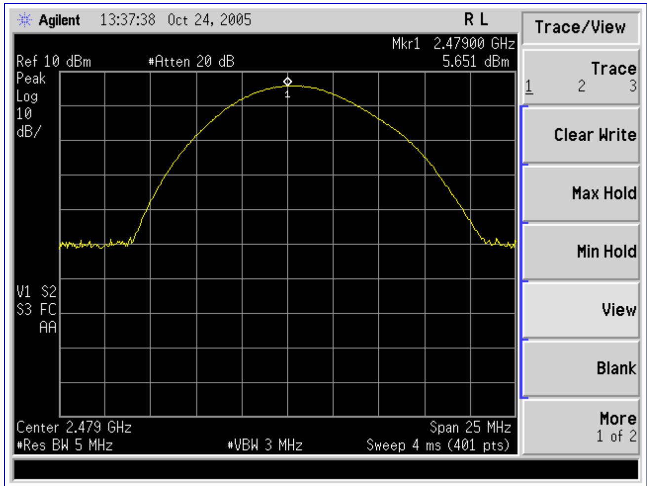
Plot 6. Peak Power Output Test Results – Channel 77
