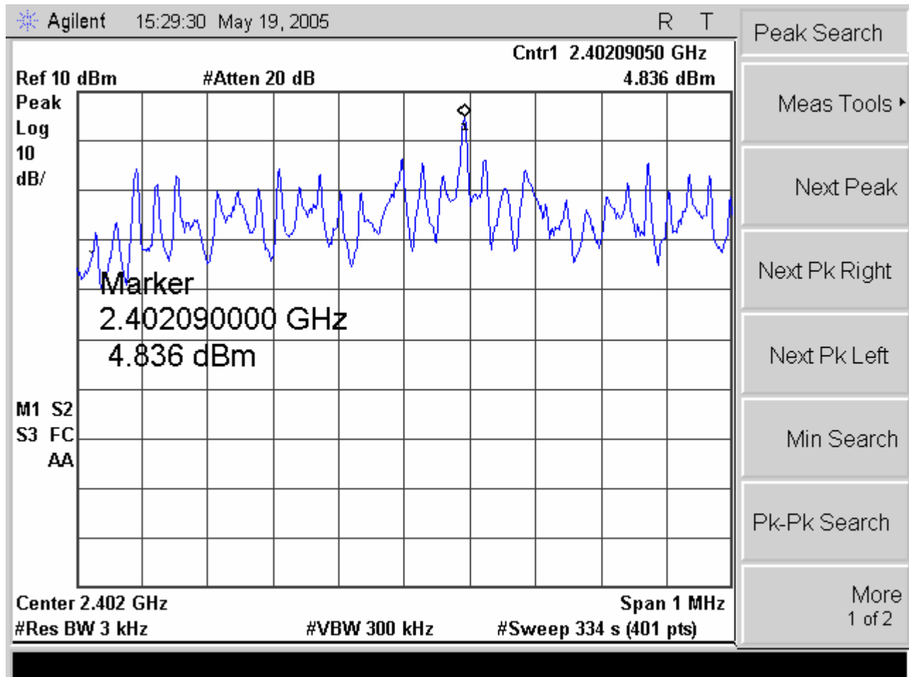
Plot 12. Power Spectral Density Test Results (Channel 0)
