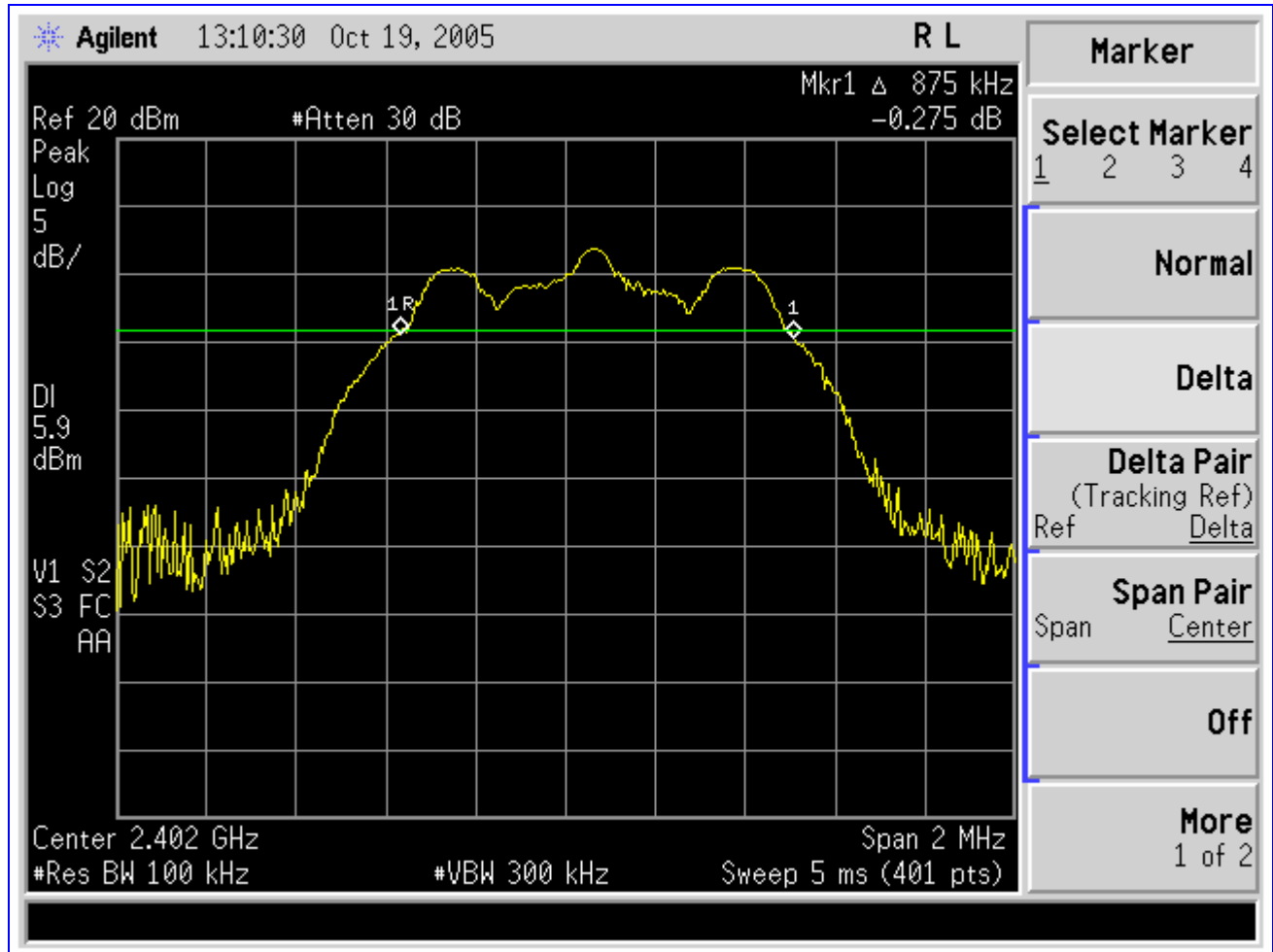
Plot 1. Occupied Bandwidth; Test Results, Channel 0
