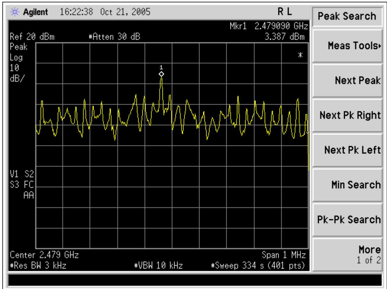
Plot 14. Power Spectral Density Test Results (Channel 77)
