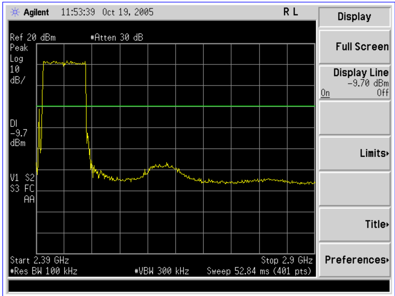
Plot 9. Spurious Conducted Emission Test Plot
