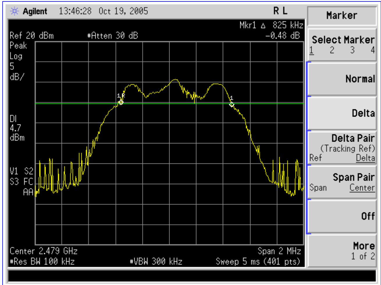
Plot 3. Occupied Bandwidth; Test Results, Channel 77
