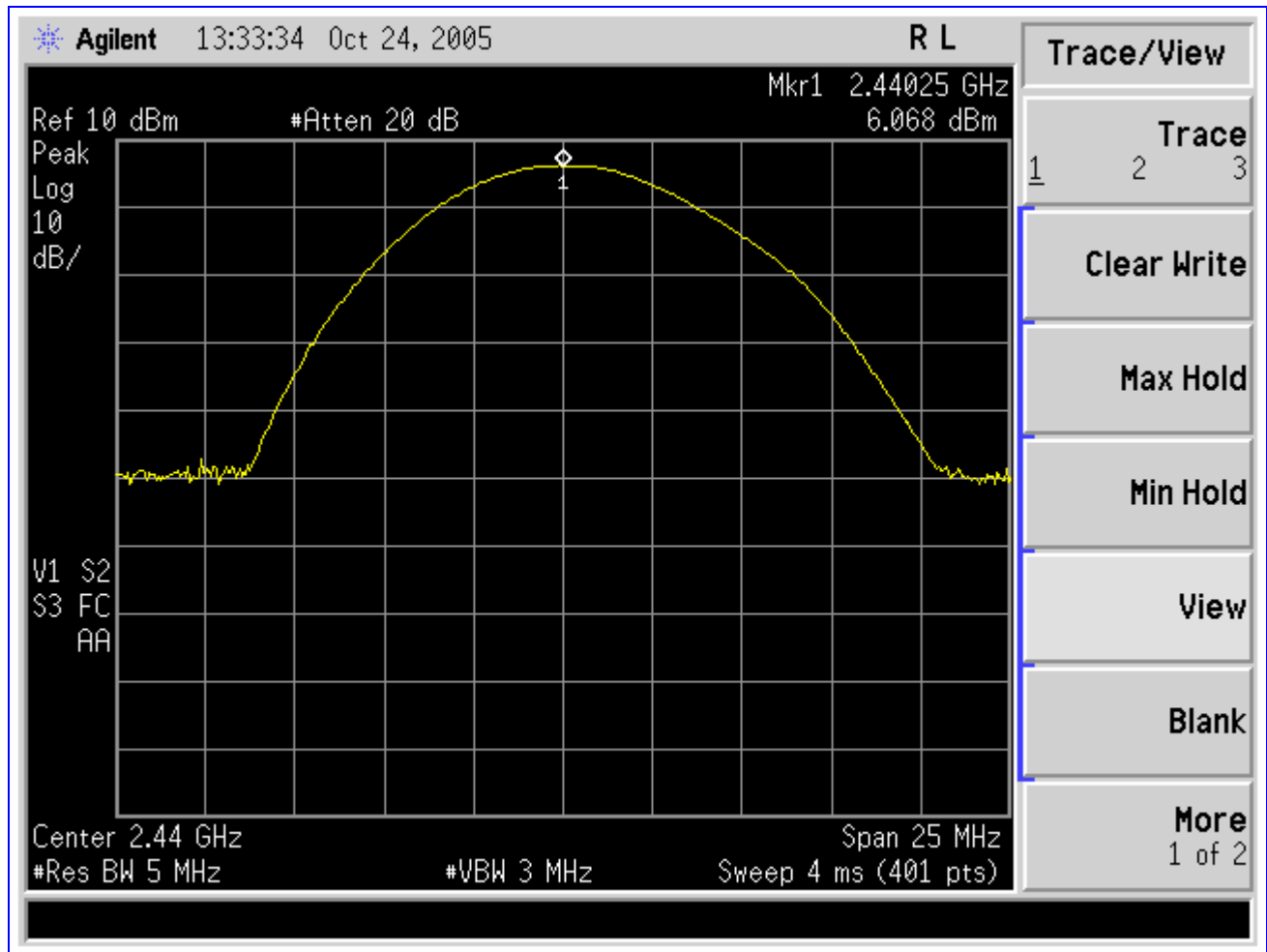
Plot 5. Peak Power Output Test Results – Channel 38
