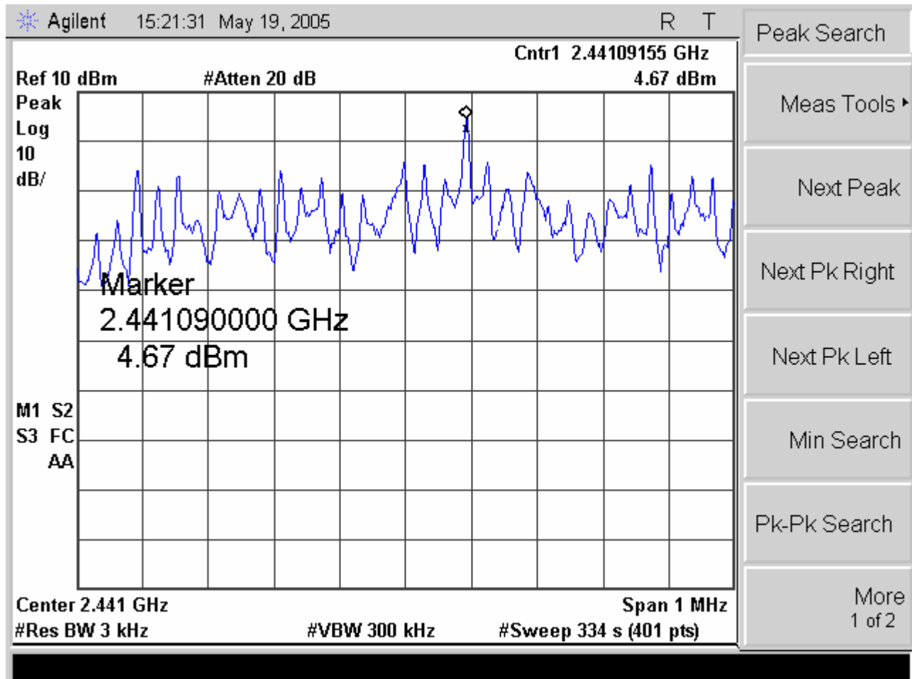
Plot 13. Power Spectral Density Test Results (Channel 39)
