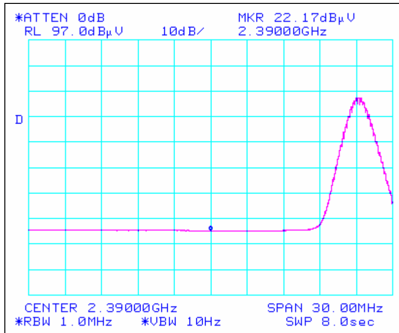
Plot 15. Band Edge Test Results, Channel Ø
