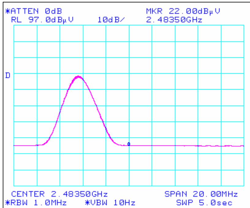
Plot 16. Band Edge Test Results, Channel 77
