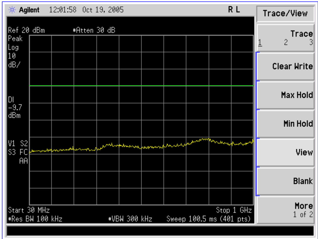
Plot 7. Spurious Conducted Emission Test Plot
