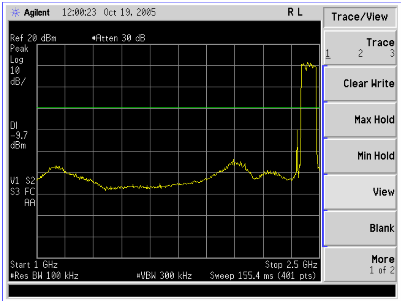
Plot 8. Spurious Conducted Emission Test Plot
