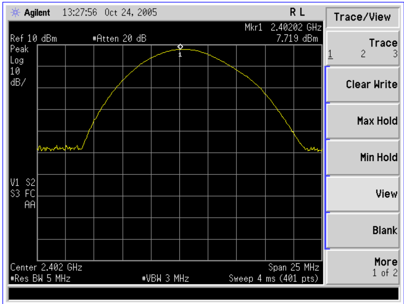
Plot 4. Peak Power Output Test Results – Channel 0
