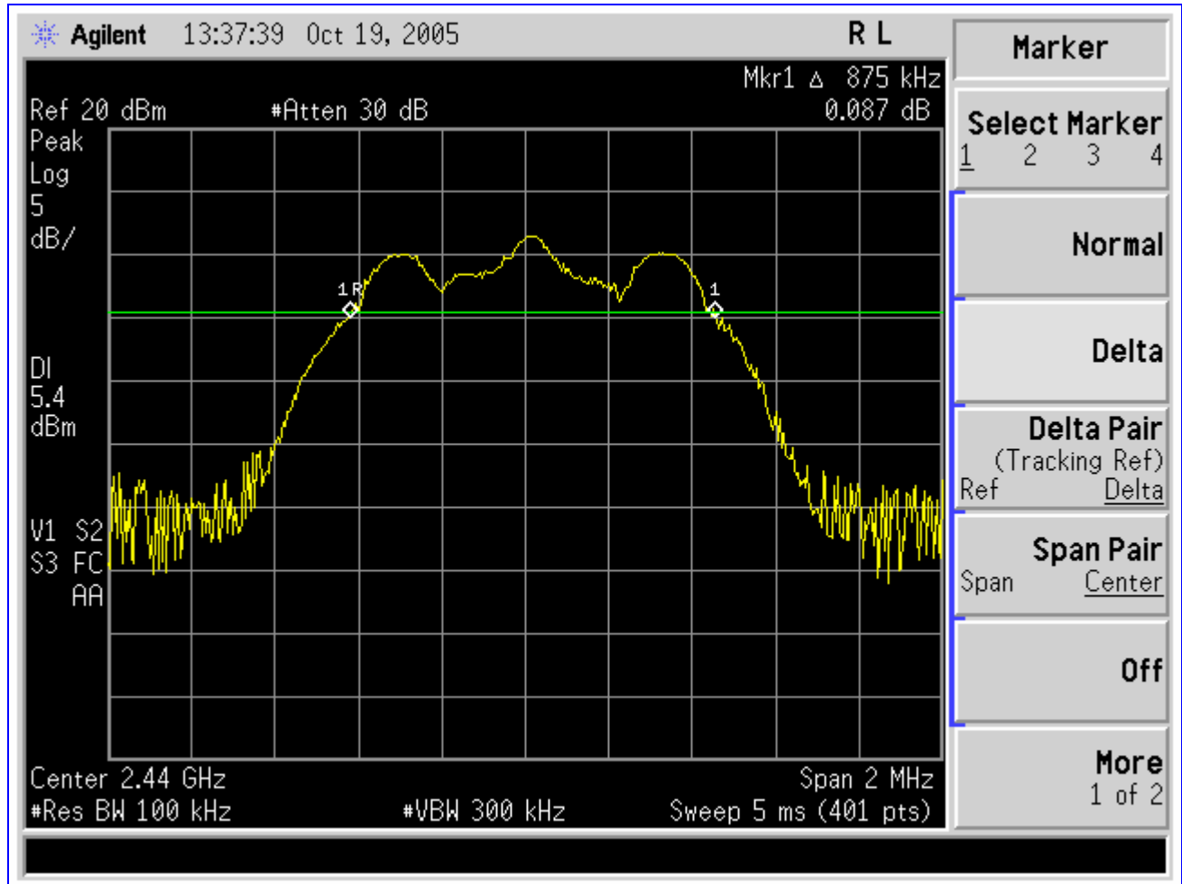
Plot 2. Occupied Bandwidth; Test Results, Channel 38 BW = 875 kHz
