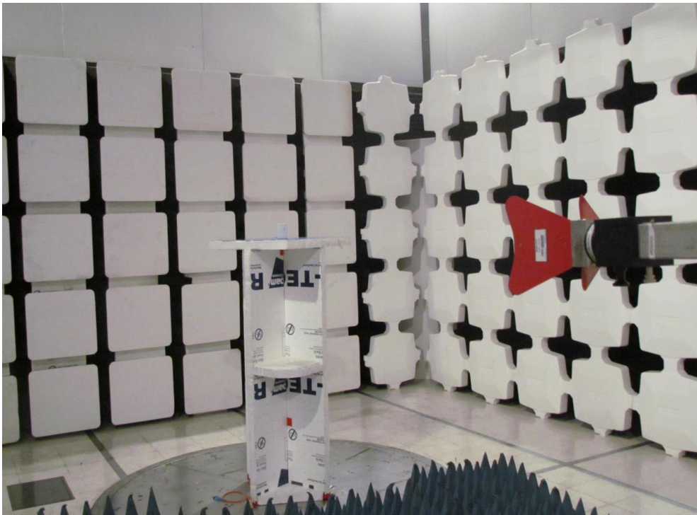
Spurious Emissions 1-18GHz
