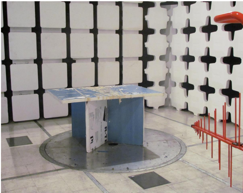
Spurious Emissions 1-18GHz
