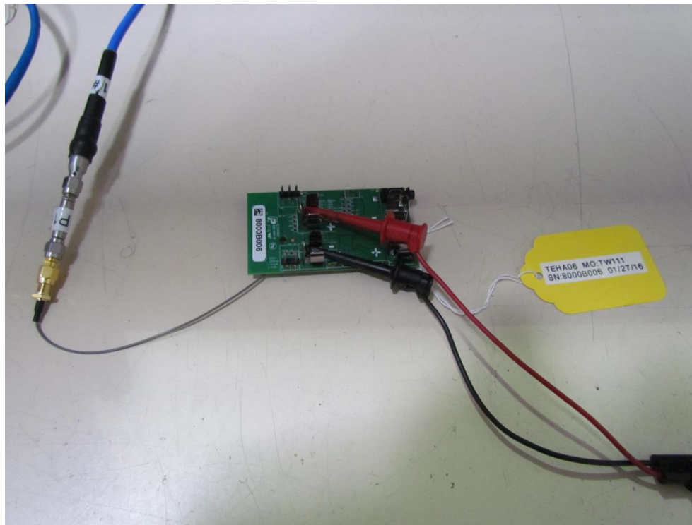
RF Conducted Test Setup #2
