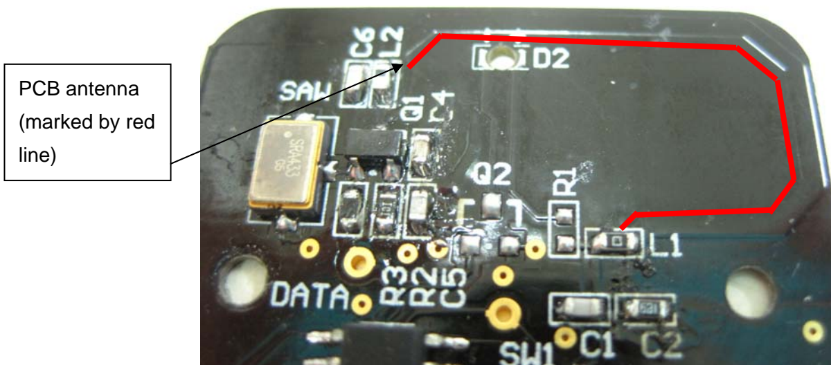
Closer view of the PCB antenna (from L2 to L1)
