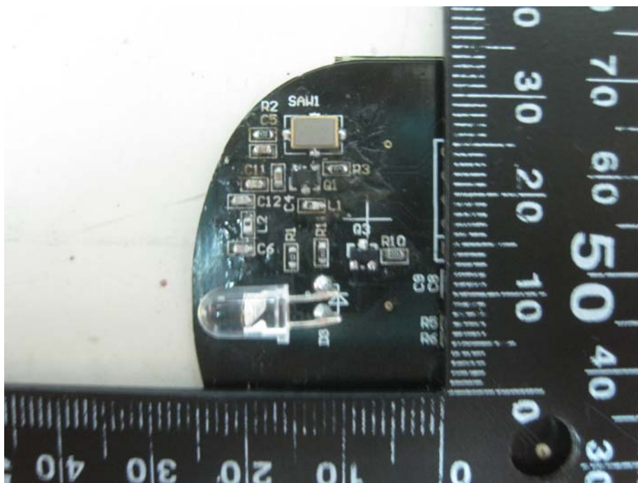
Closer view of the RF module
