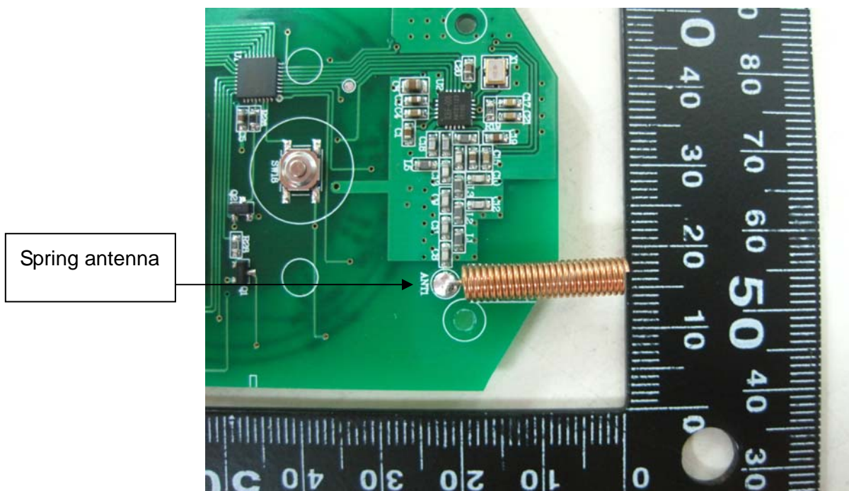
Closer view of the PCB antenna
