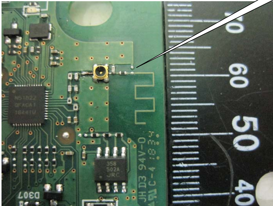
Closer View of the PCB ANT
