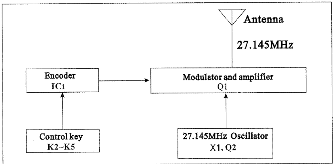
transmitter block diagram
