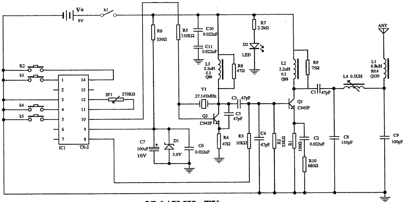
27.145MHz TX
