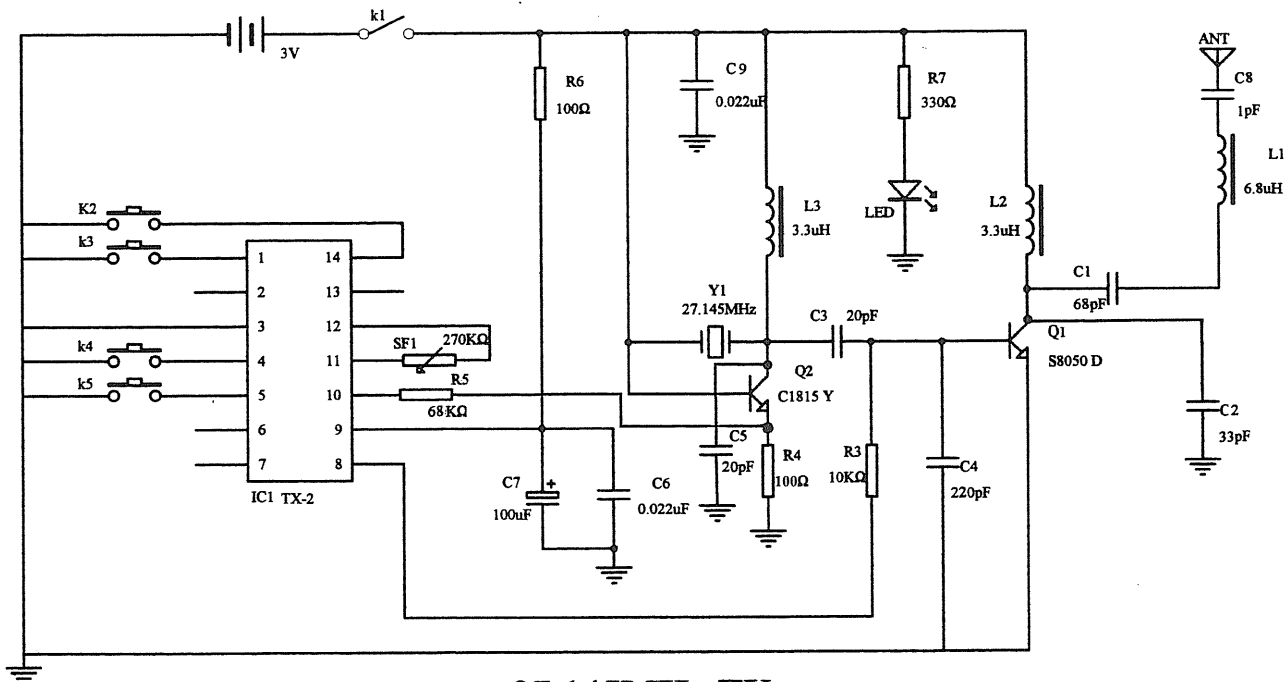
27.145MHz TX
