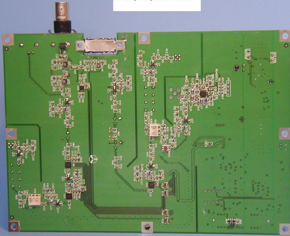
RF Card, back, shield removed
