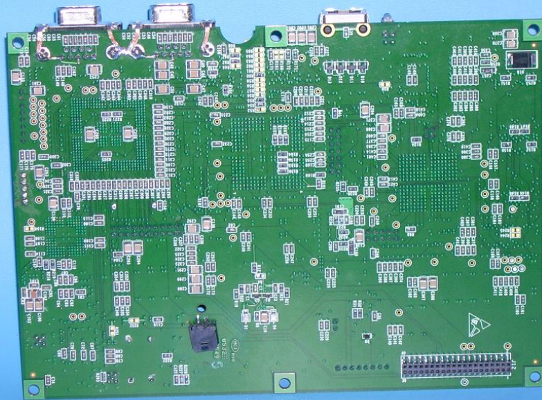
Digital Board, bottom
