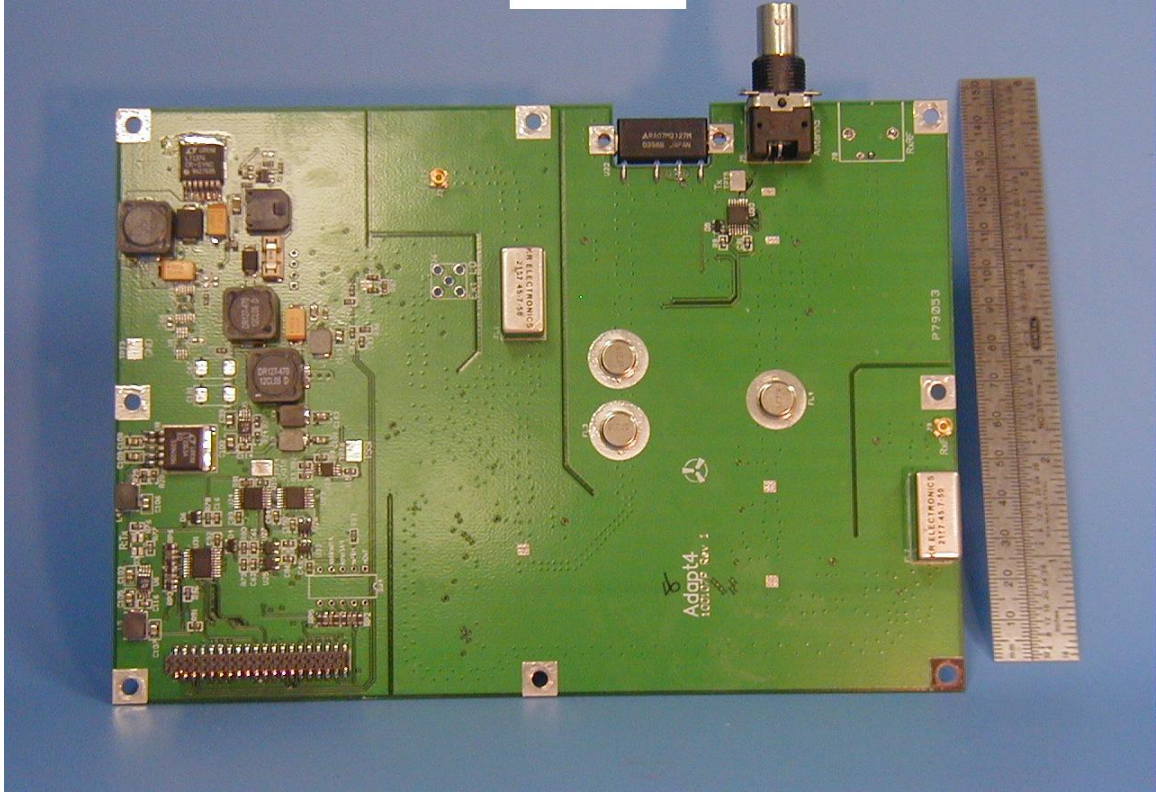
RF board, top
